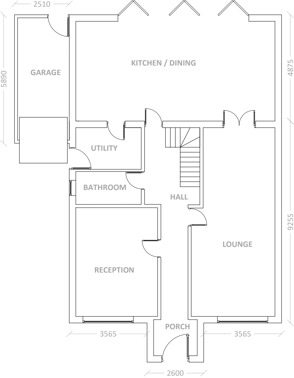
PROPOSED GF PLAN 1:100
