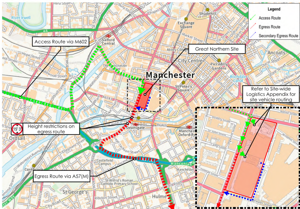
Figure 07 – HGV Construction Access (shown dotted green) and Egress Route (shown dotted red and blue)
