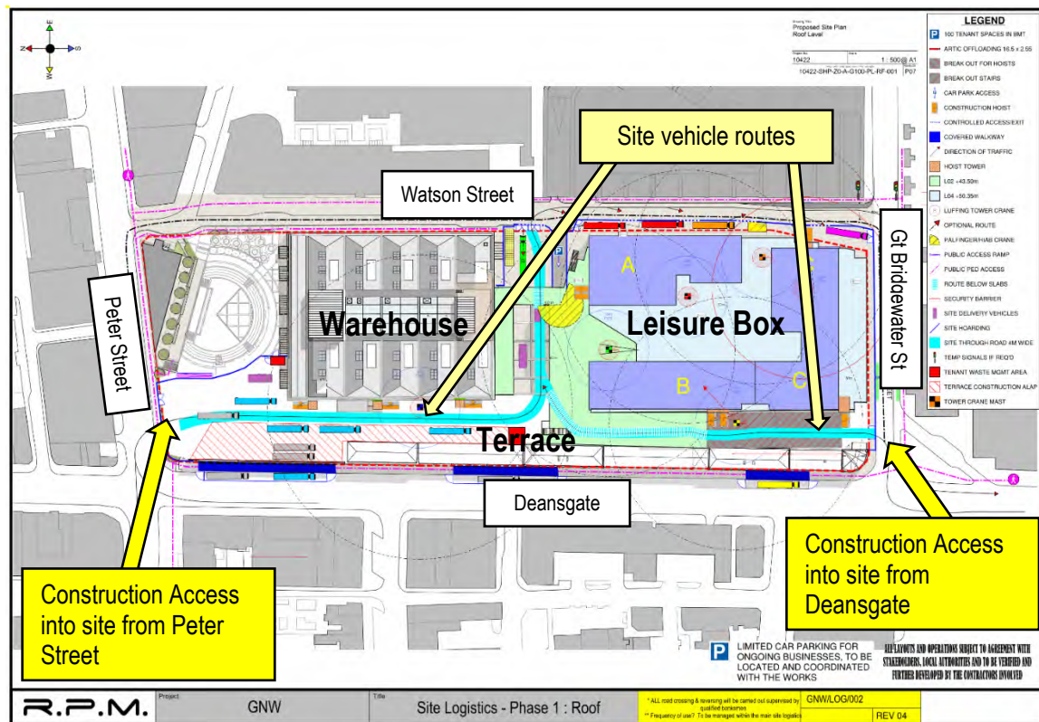
Figure 06 – Logistics Extract Plan indicating Site Construction Vehicle Access points and Site Routes
