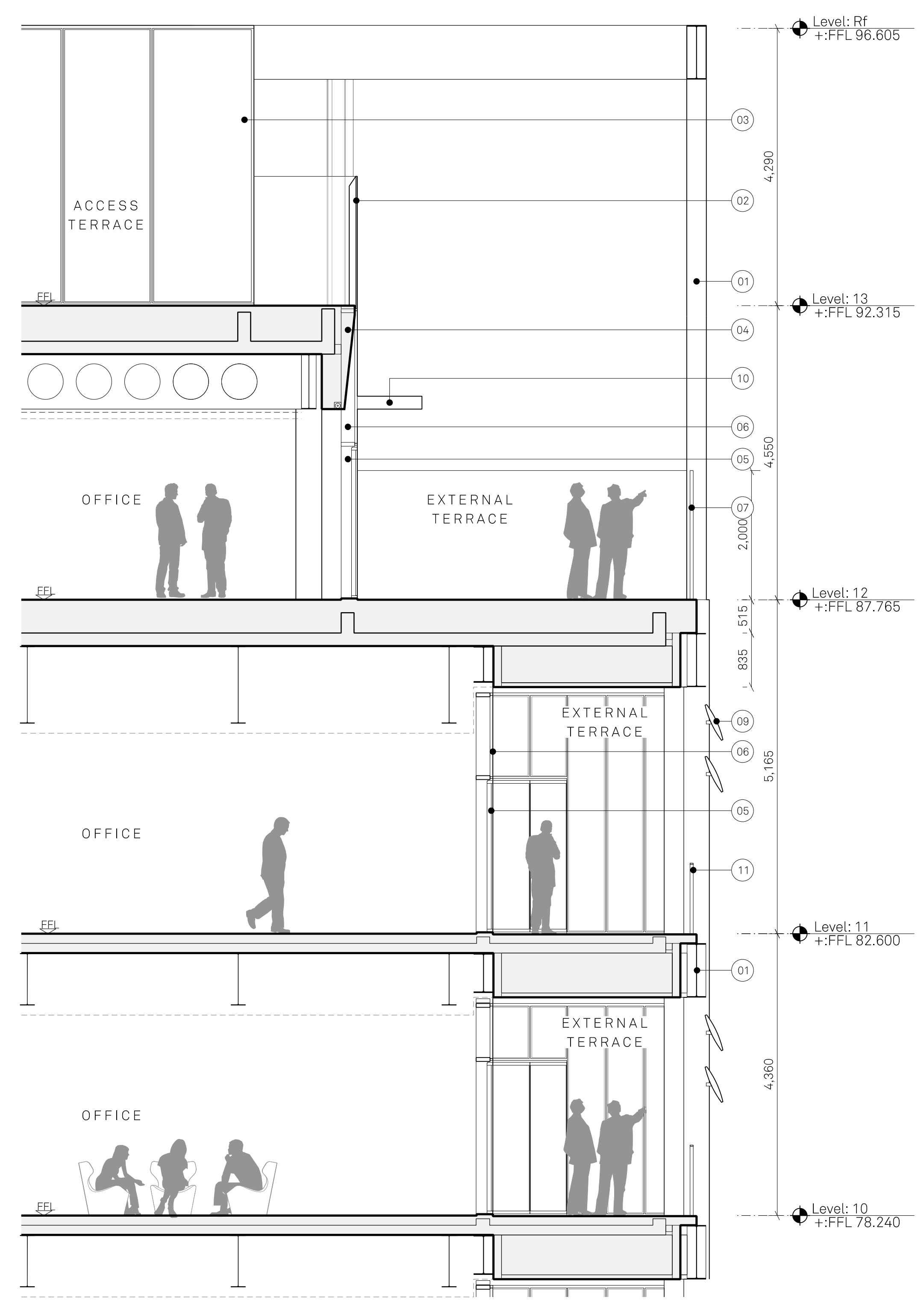
SECTION AA Typical Floor through External Terraces
