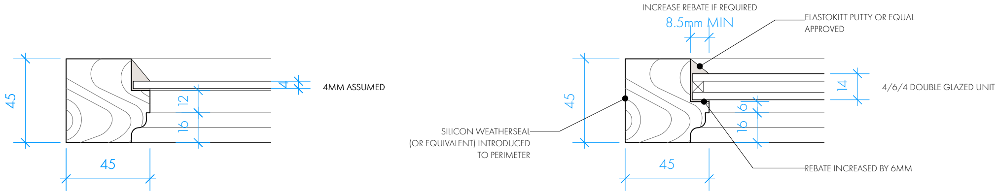
01_INCREASE IN REBATE DETAIL EXISTING CASEMENT TYPICAL 1:2@A3
