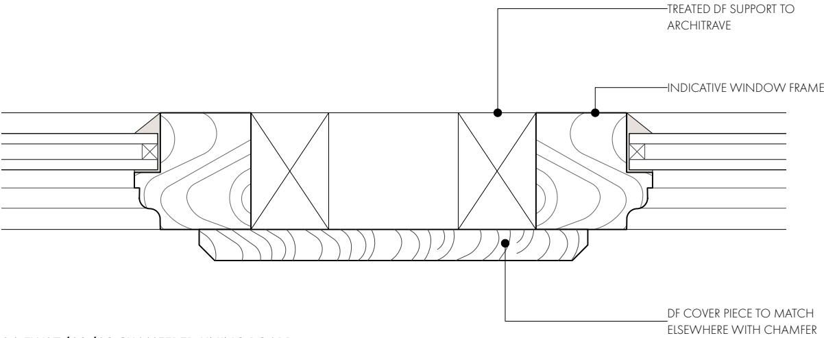
04_EW07/08/09 CHAMFERED LINING BOARD 1:2@A3
