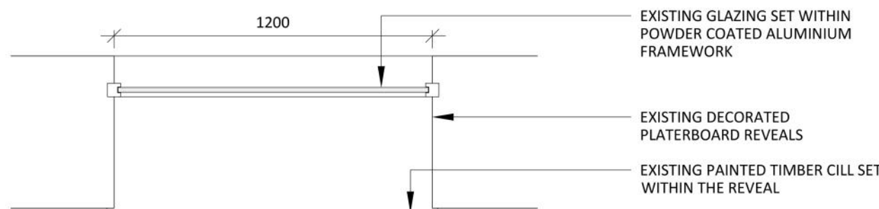
02 THIRD FLOOR EXISTING WINDOW PLAN SCALE - 1:20 @ A1 DETAIL PLAN
