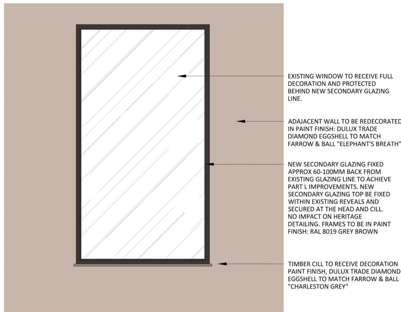
04 THIRD FLOOR PROPOSED WINDOW ELEVATION SCALE - 1:20 @ A1 DETAIL ELEVATION
