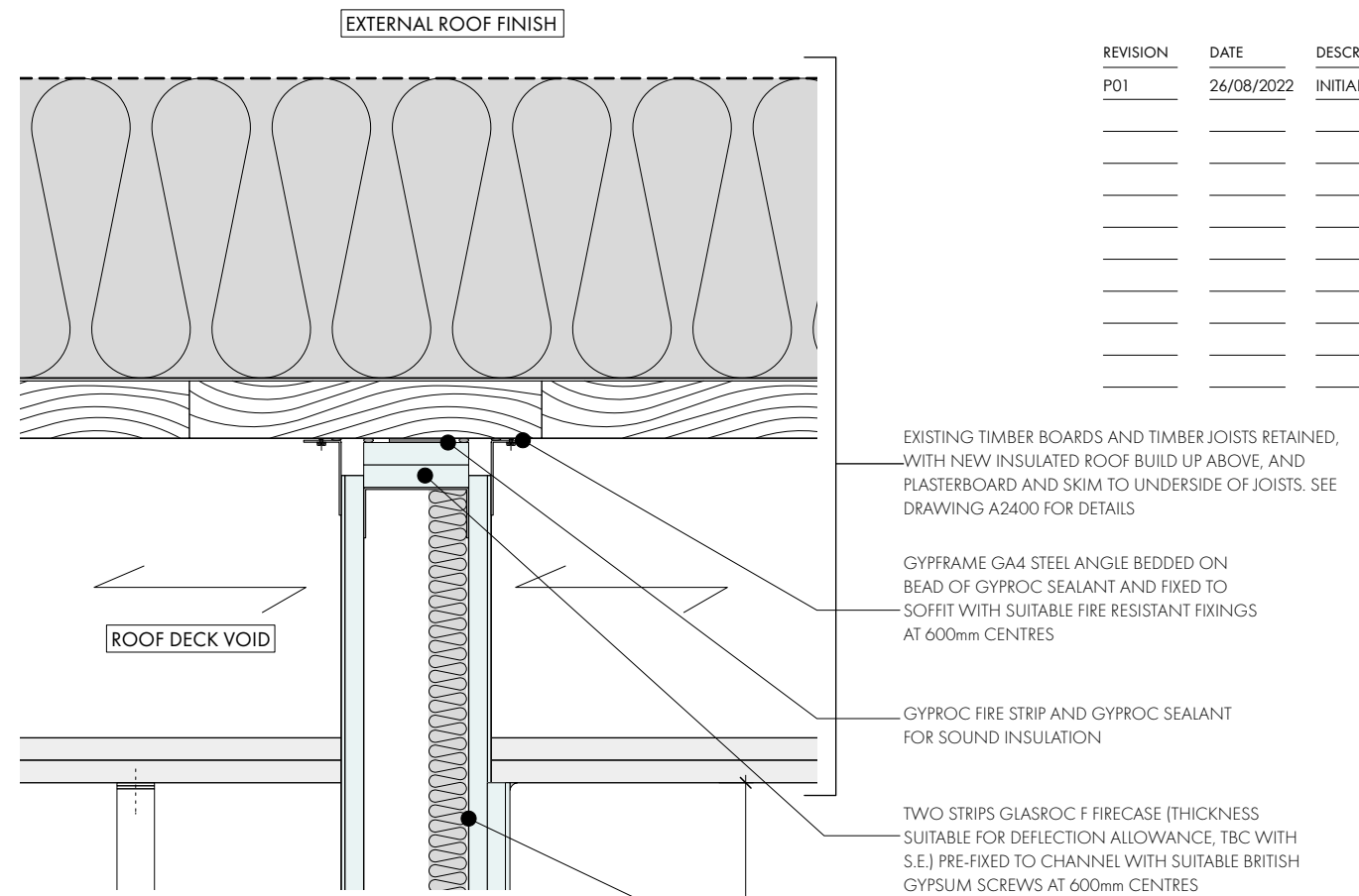
DETAIL 04 - TOP OF L02 PARTITION DEFLECTION HEAD
