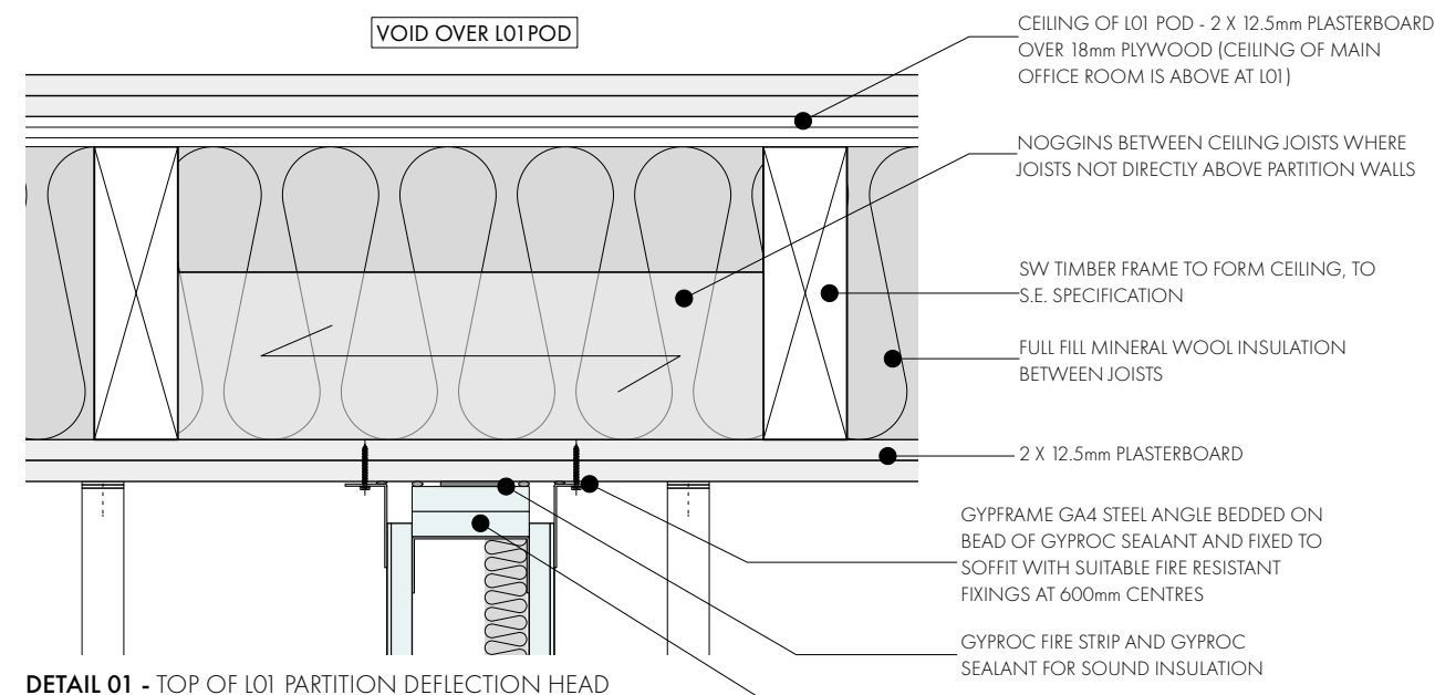
DETAIL 01 - TOP OF L01 PARTITION DEFLECTION HEAD
