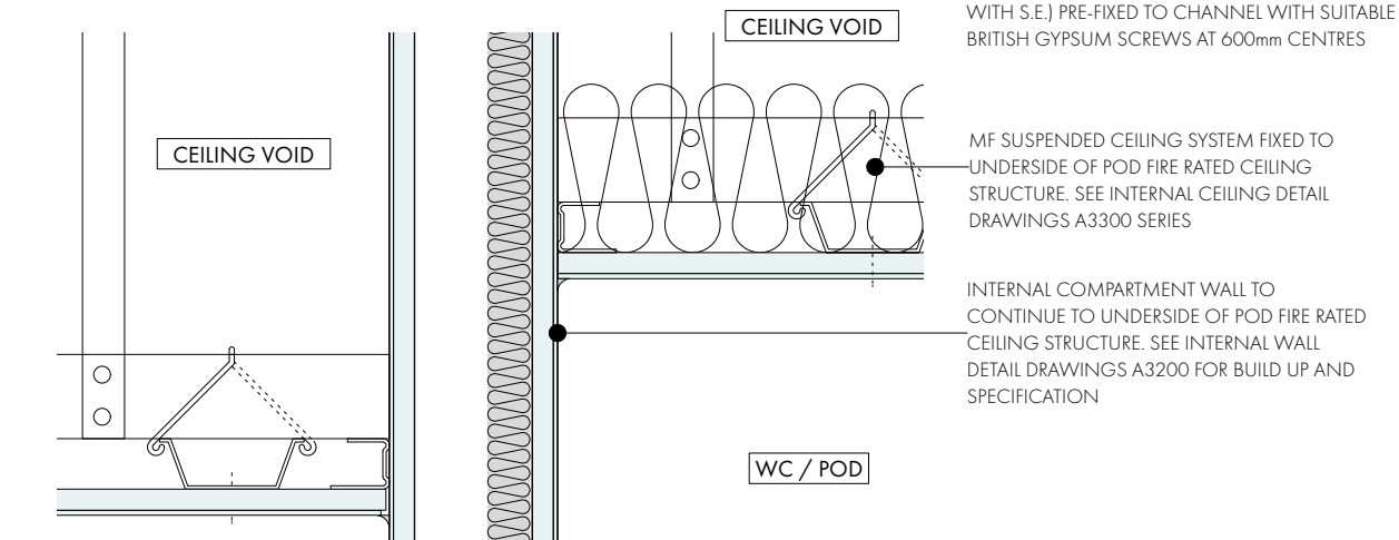
DETAIL 02 - POD CEILINGS
