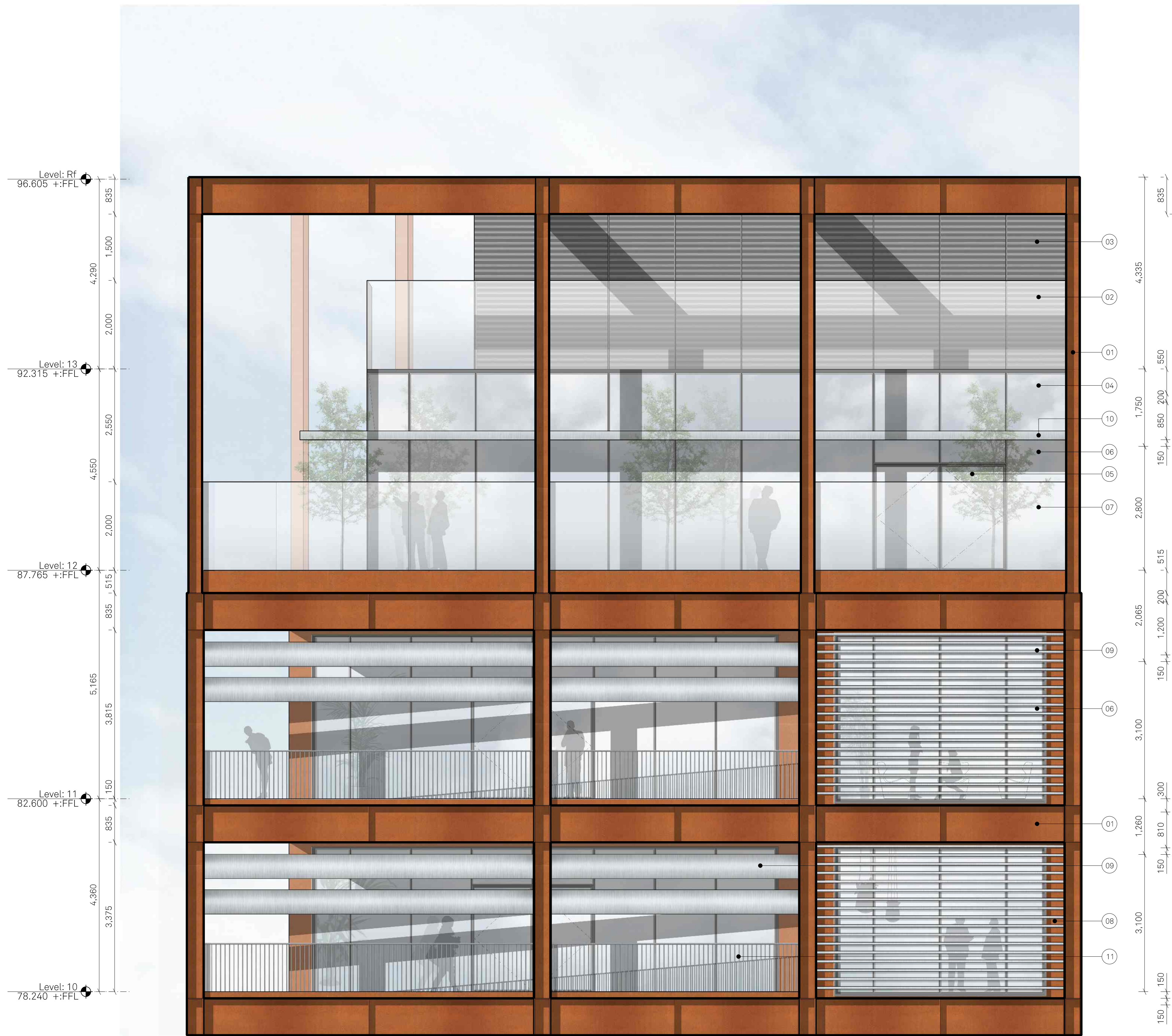
PARTIAL ELEVATION Medlock Junction External Balcony
