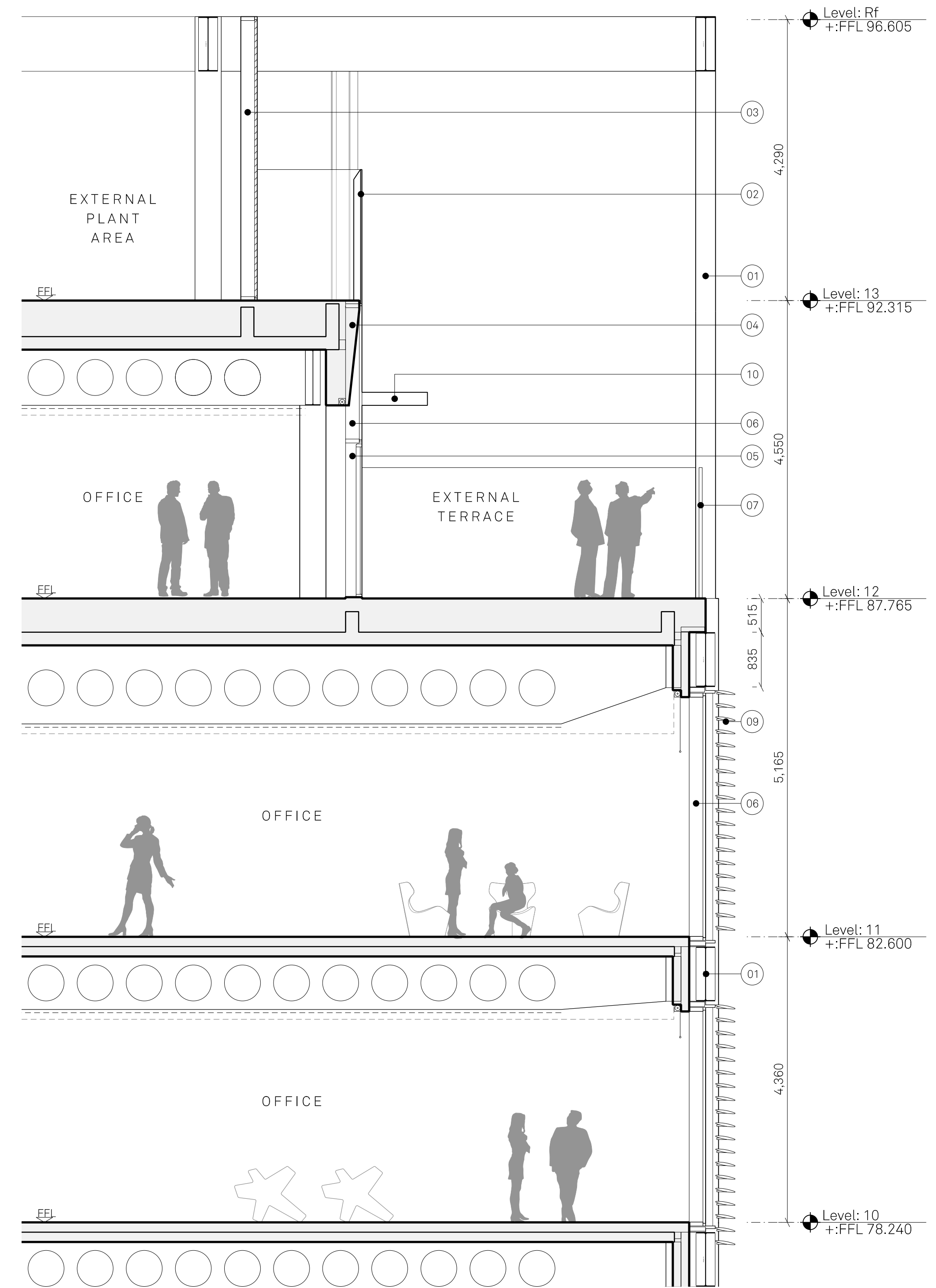
SECTION AA Typical Floor With Louvre Shading & Roof Terrace
