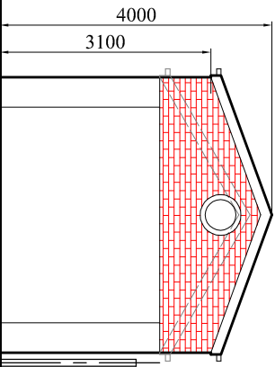
PROPOSED FRONT ELEVATION
