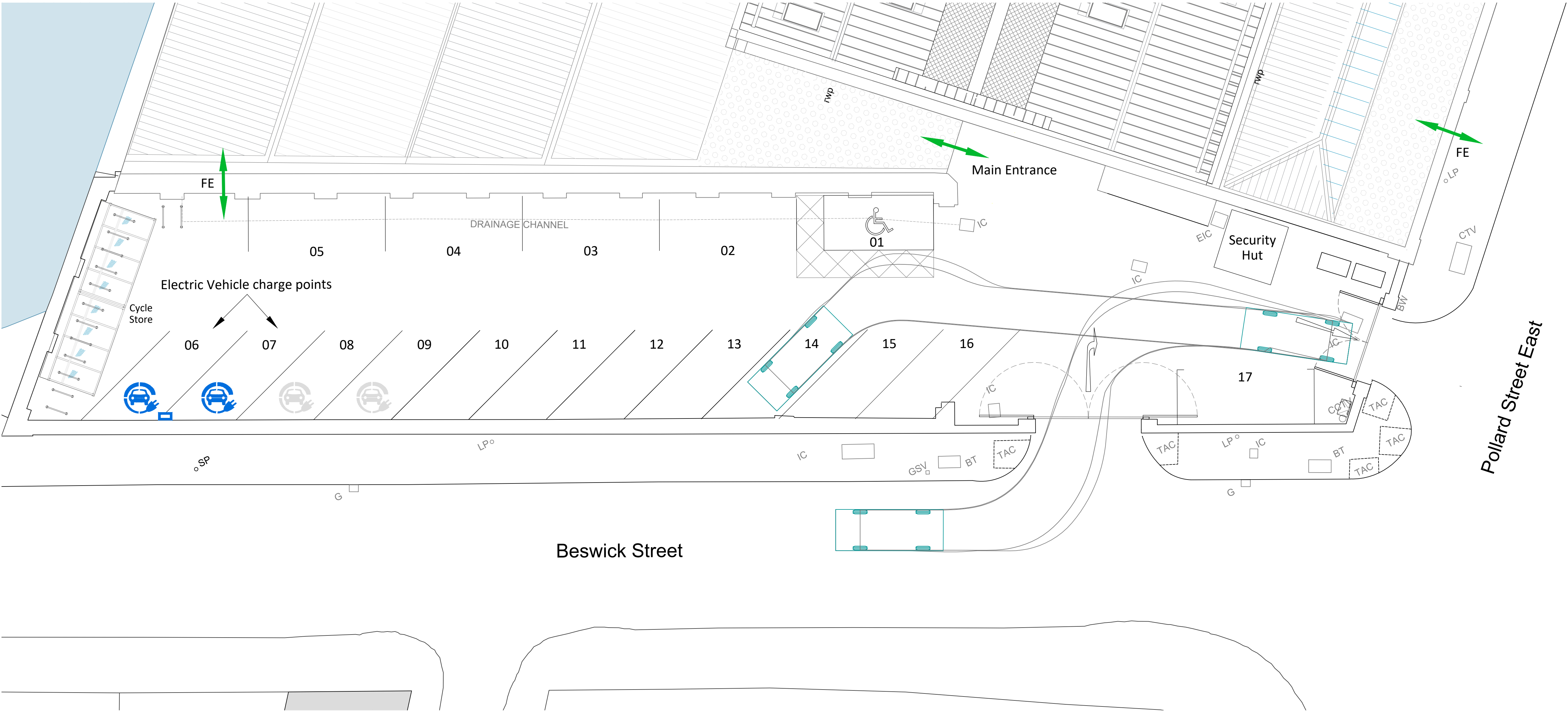
Existing Parking Plan Scale 1:100 Scale Bar 1:100 @ A1
