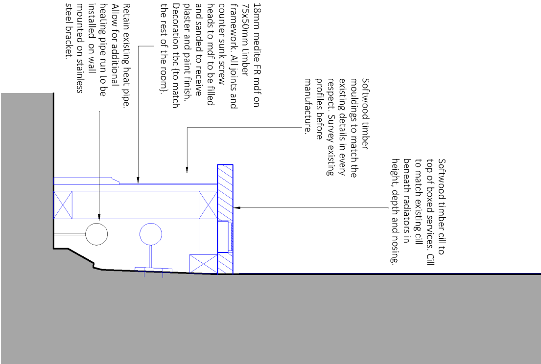
Proposed Detail F - Heating Service Boxing - Wall and Skirting Detail
