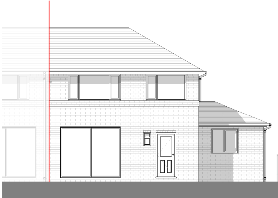
Rear Elevation 1 : 100
