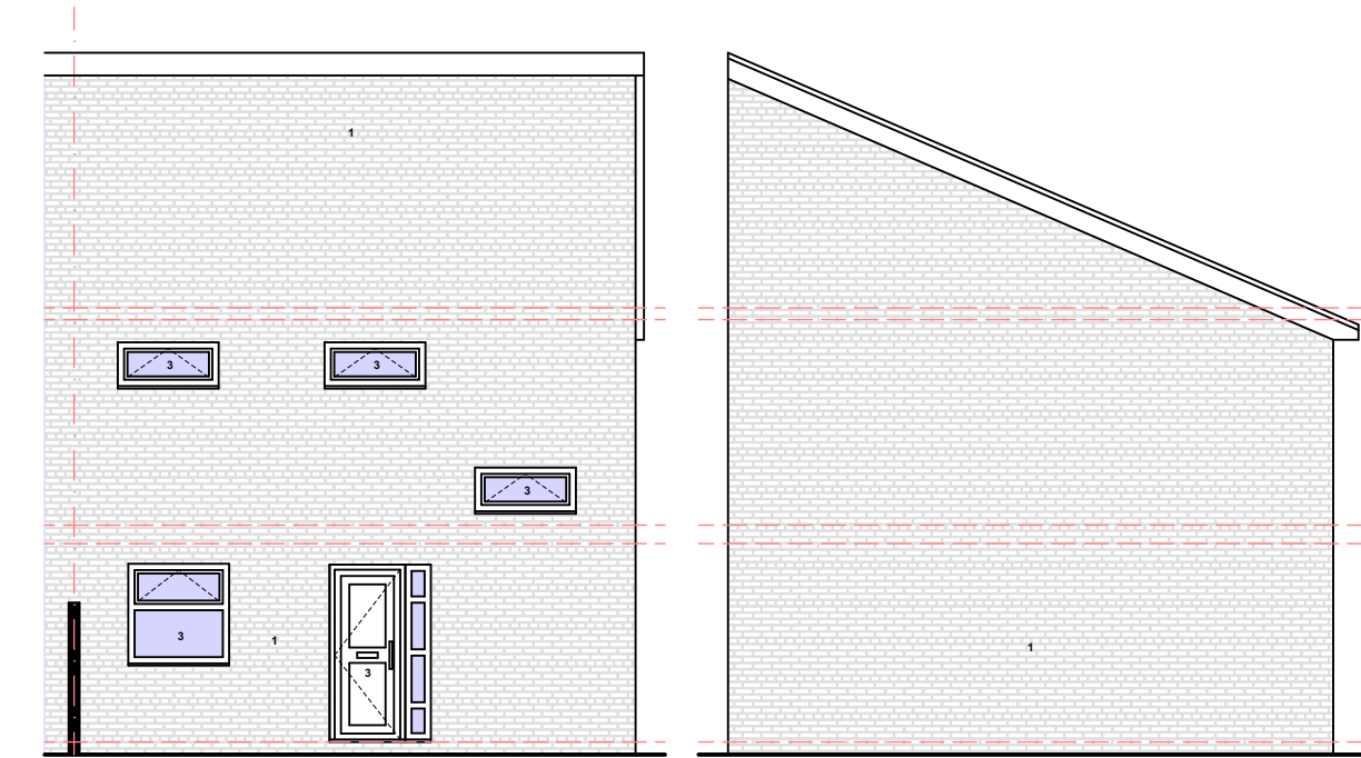
EXISTING GA FRONT ELEVATION @1:100
