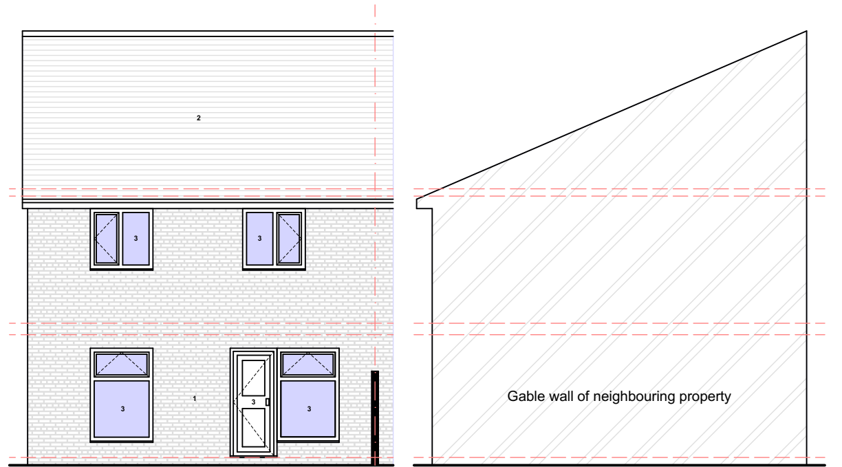
EXISTING GA REAR ELEVATION @1:100
