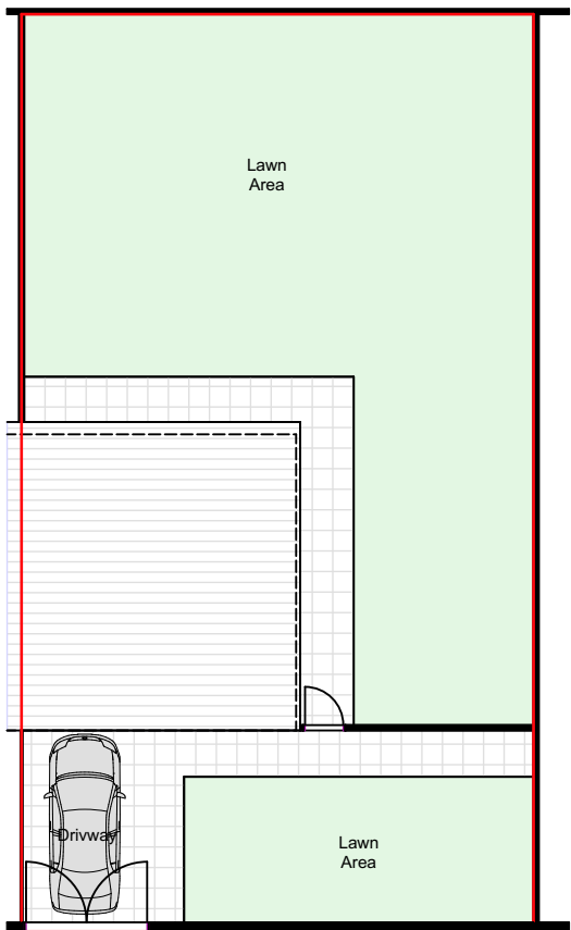
EXISTING GA SITE PLAN @1:200
