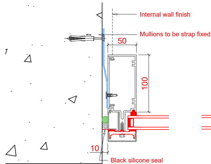
02 CW L/H Mullion Detail - G Scale 1:4
