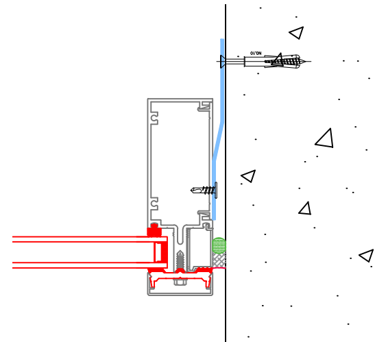
02 CW R/H Mullion Detail - L Scale 1:4
