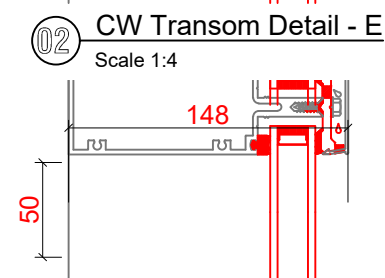
02 CW Transom Detail - E Scale 1:4
