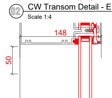
02 CW Transom Detail - E Scale 1:4
