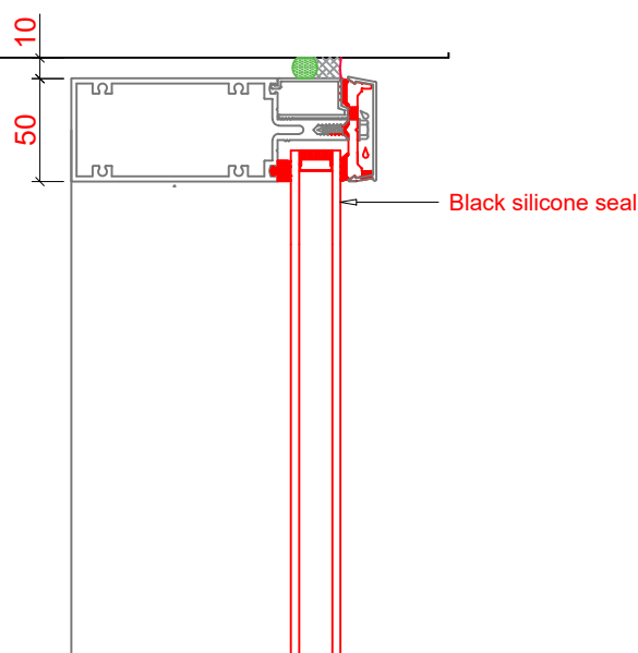
02 CW Head Transom Detail - D Scale 1:4
