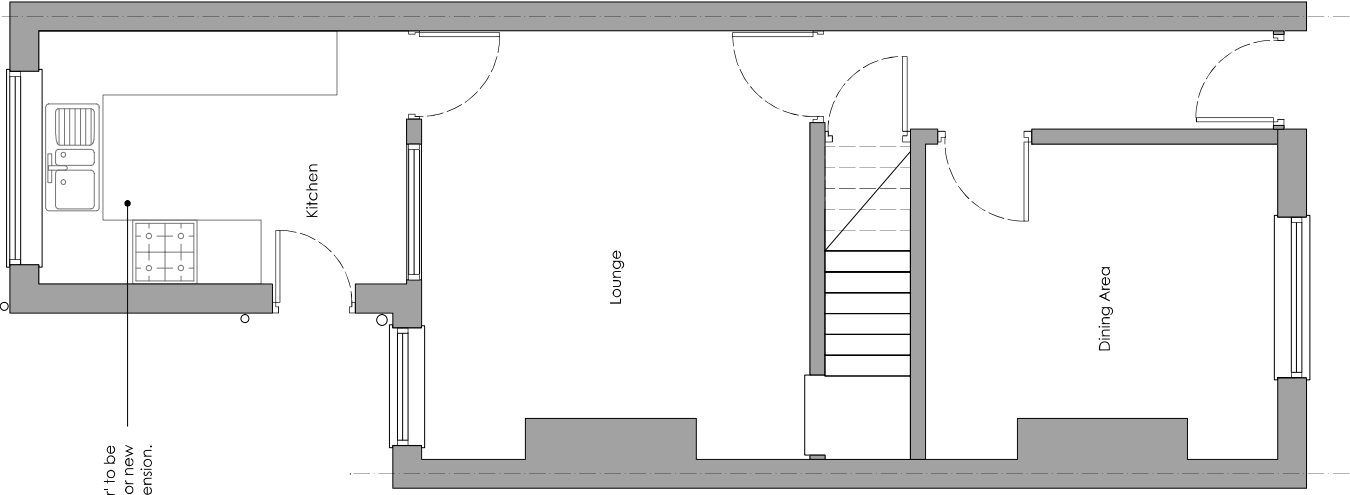
Existing Ground Floor Plan 1:50
