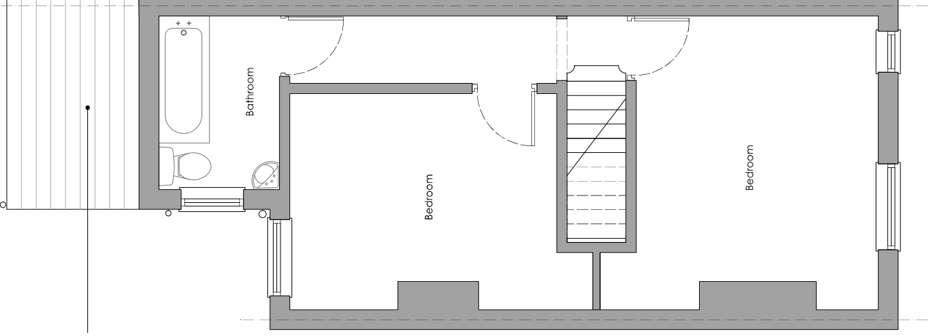
Existing First Floor Plan 1:50
