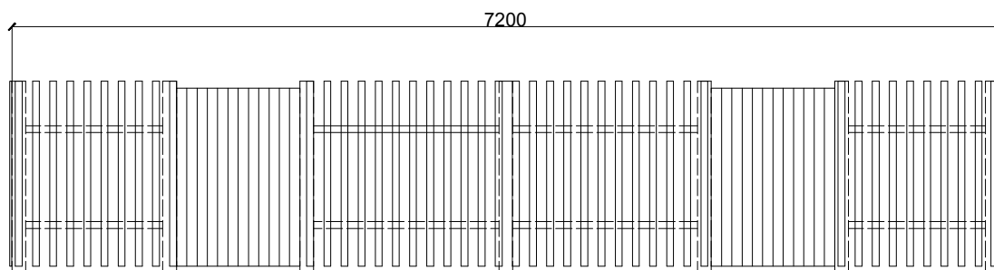
BIN STORE PLAN
