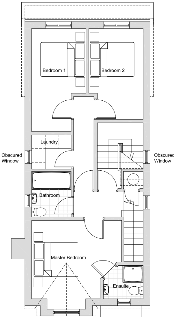
Proposed 1/F Plan 1:100
