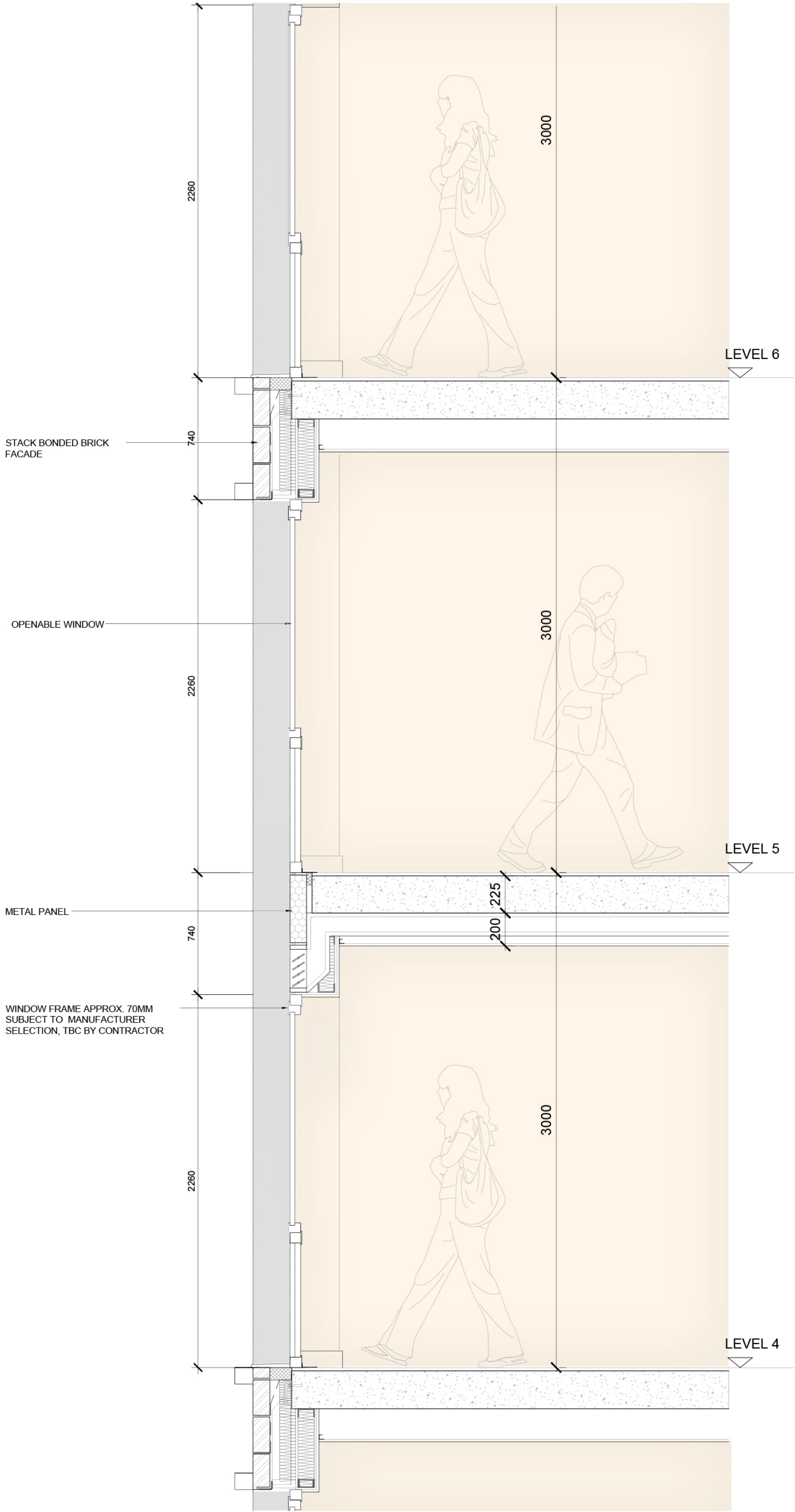
EXTERNAL WALL DETAIL SECTION STANDARD WINDOW BAY
