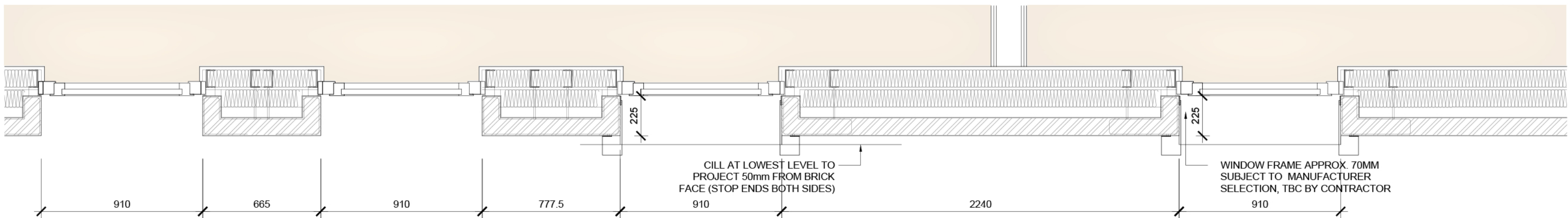
EXTERNAL WALL DETAIL PLAN STANDARD WINDOW BAY
