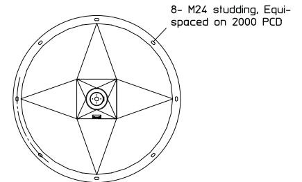
Plan View on RRB
