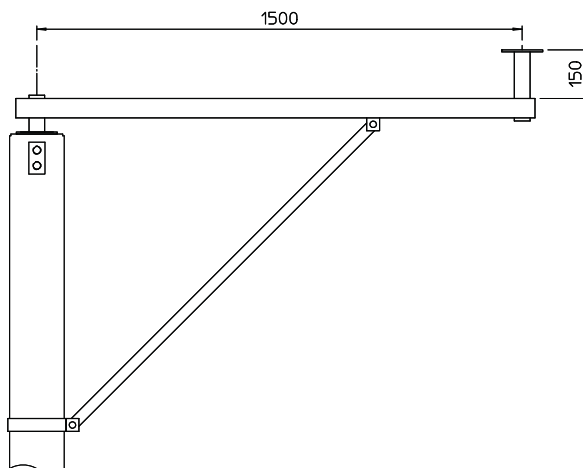
Tubular Offset Bracket for PTZ
