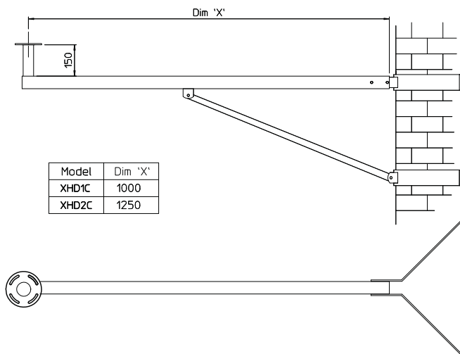
corner mount
