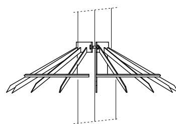
ACB3/ ..... (state Section) Anti Climb Guard Square Columns
