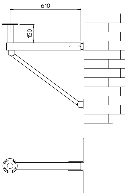
HDPTW Wall mount
