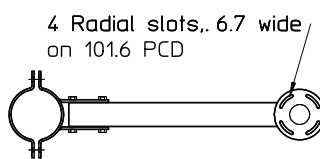
Tubular Offset Bracket for PTZ
