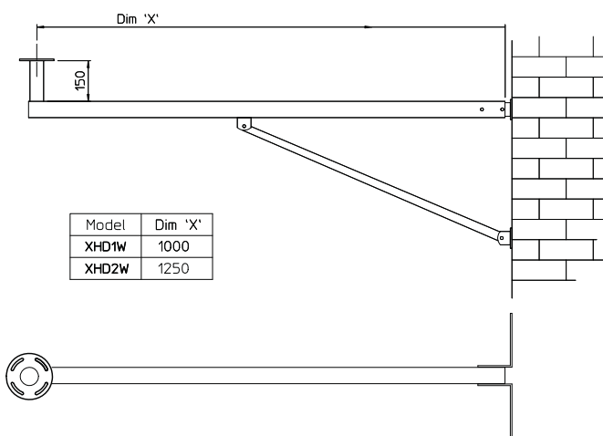
Wall mount
