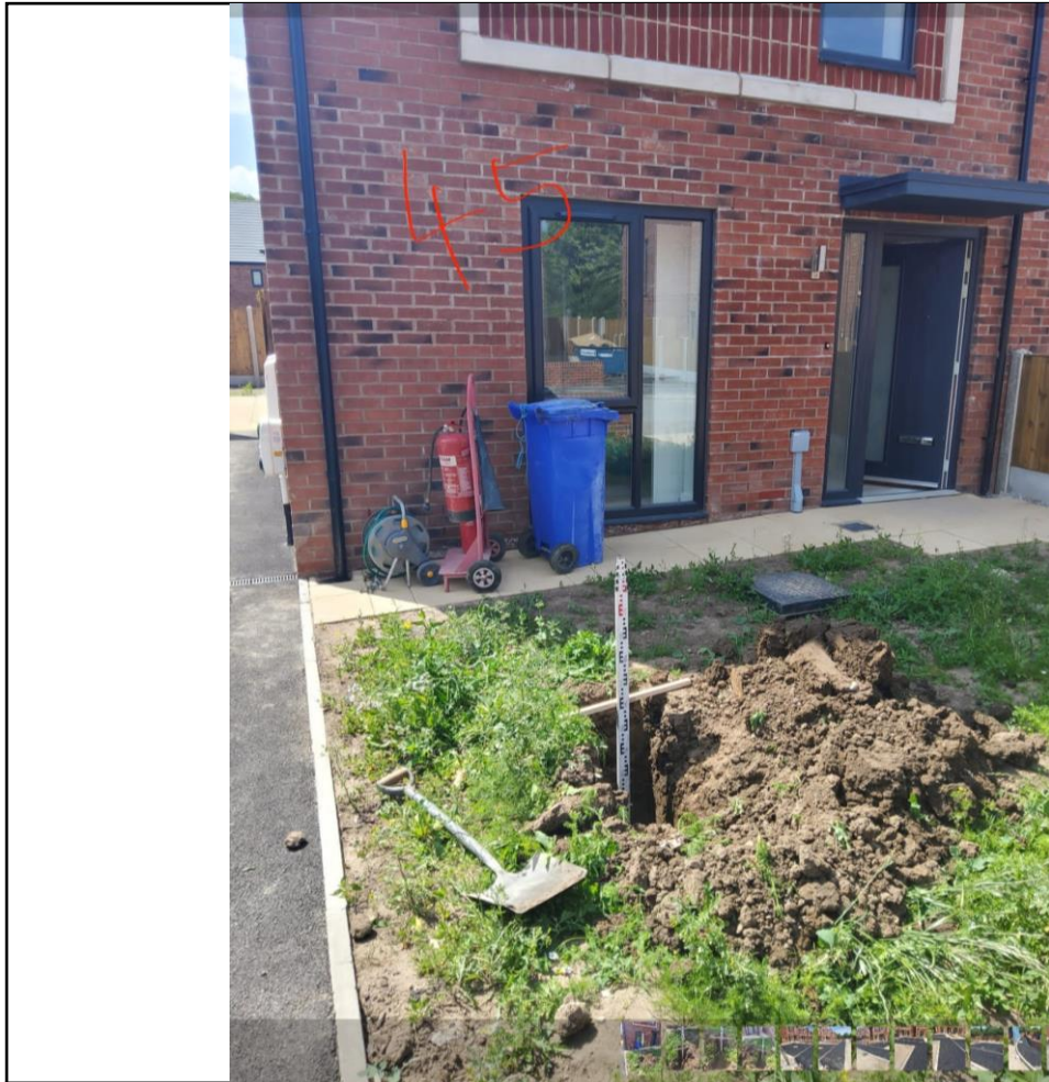
Photograph 22: Trial pit showing 600mm capping overlying high-visibility membrane in front garden area of plot 45.
