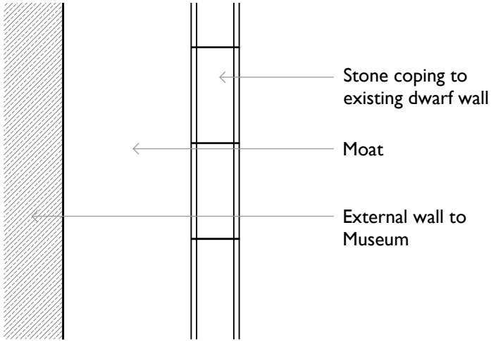
1 1207 Copings as Existing 1:50 @ A4
