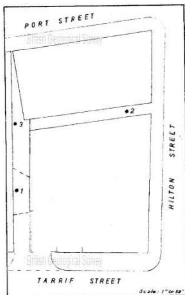
BOREHOLE LOGS & PRESSUREMETER TESTS HILTON STREET MANCHESTER
