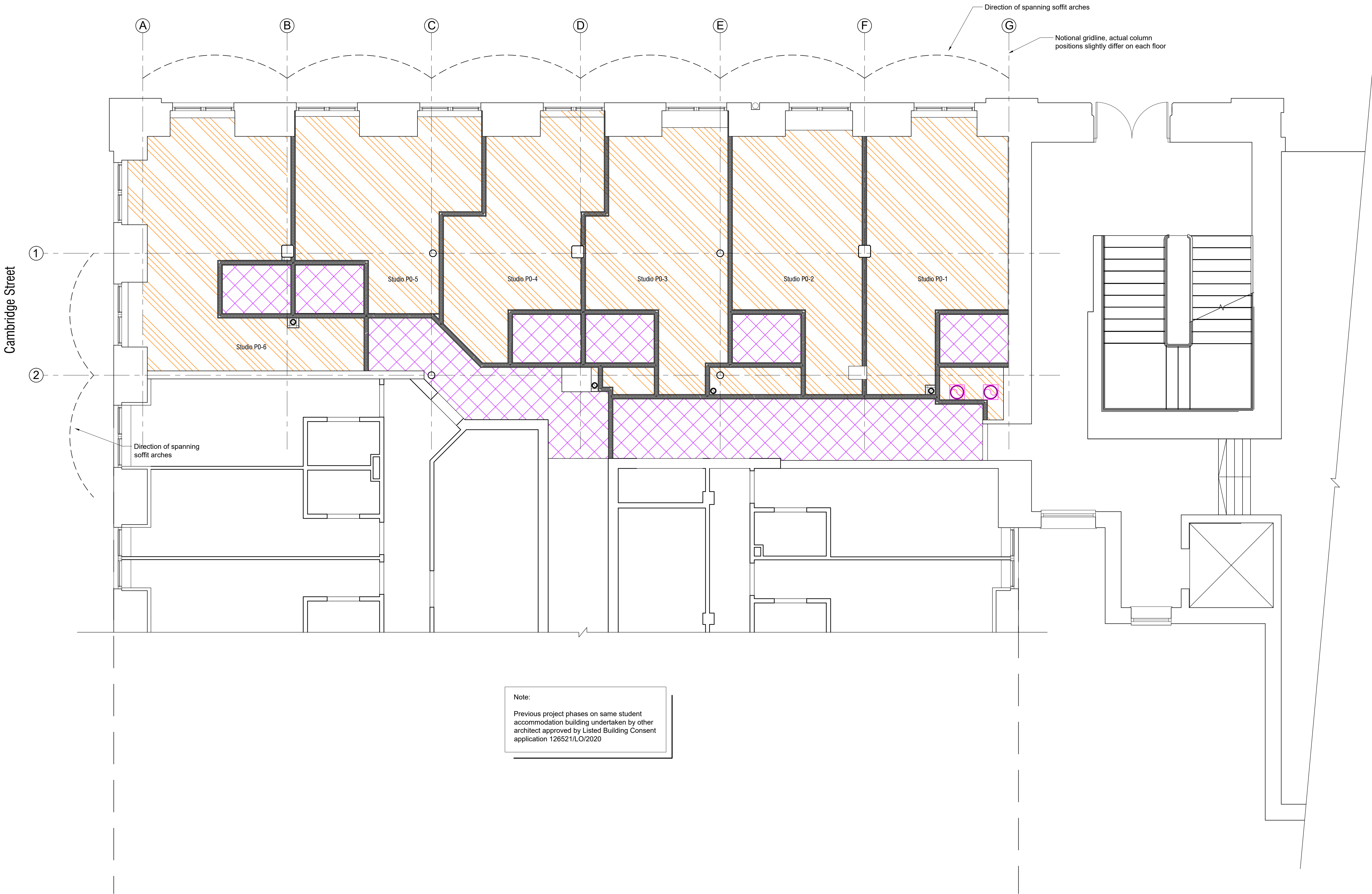
Proposed Ground Floor Ceiling [Level 0] Typical Ceiling Plan Scale 1:50
