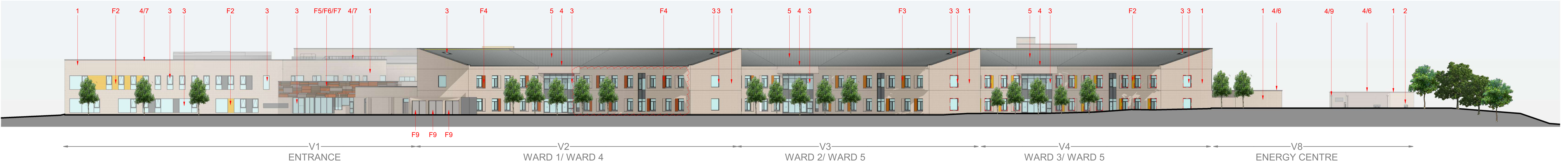
① ZZ-05_20-ZZ-9004_Elevation NW 1 : 250
