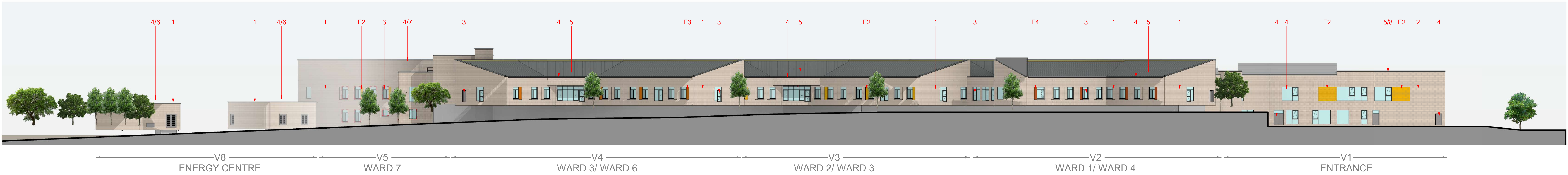
④ ZZ-05_20-ZZ-9002_Elevation SE 1 : 250
