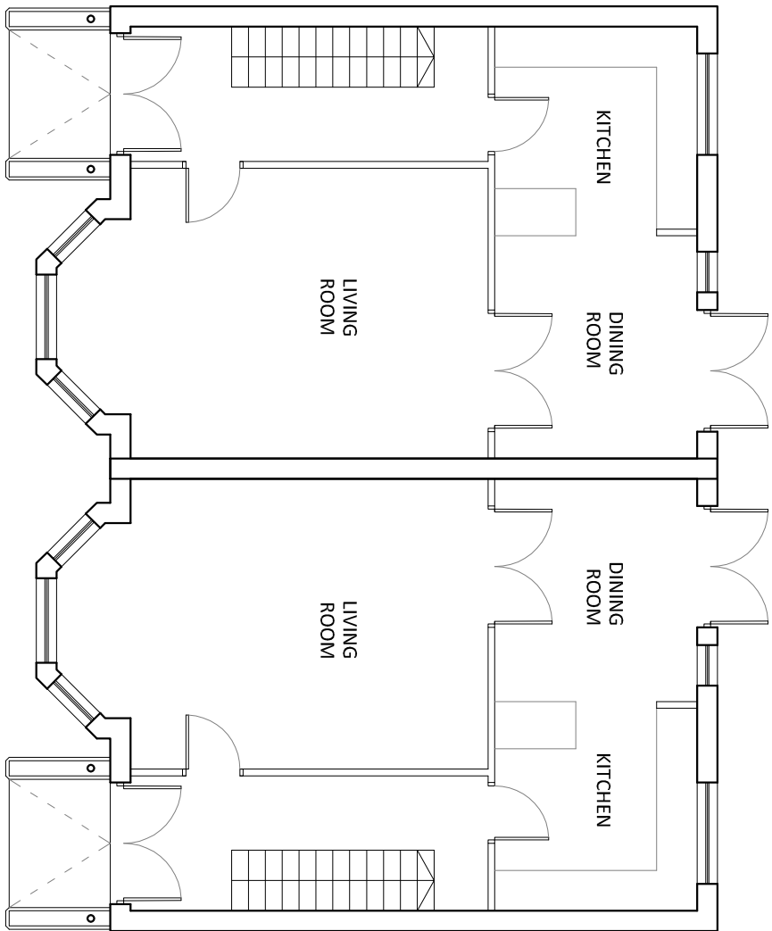
ENTRANCE LEVEL PLAN
