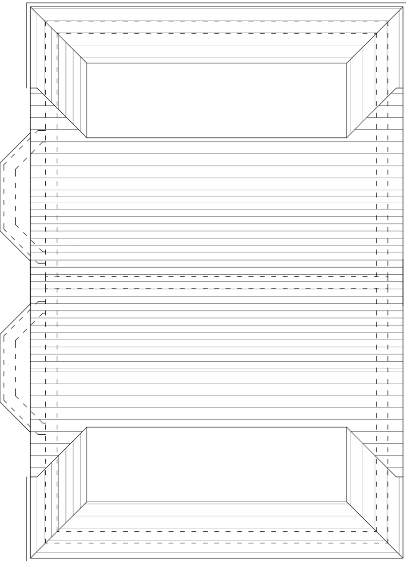
ROOF PLAN
