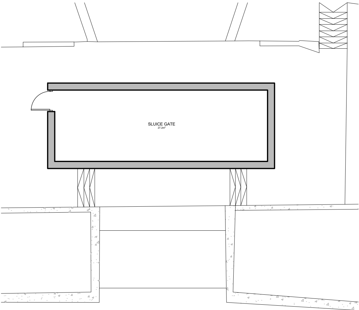
EXISTING GROUND FLOOR PLAN Scale - 1:100 @ A1
