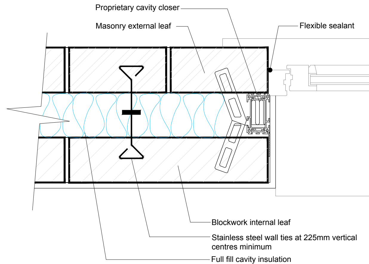
BRICK AND BLOCK WALL CONSTRUCTION, WINDOW REVEAL DETAIL - 1:5
