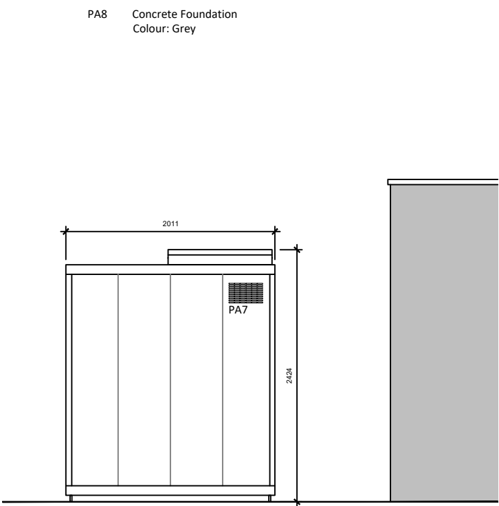
PROPOSED ELEVATION D SCALE 1:50
