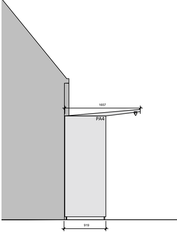
PROPOSED ELEVATION B SCALE 1:50
