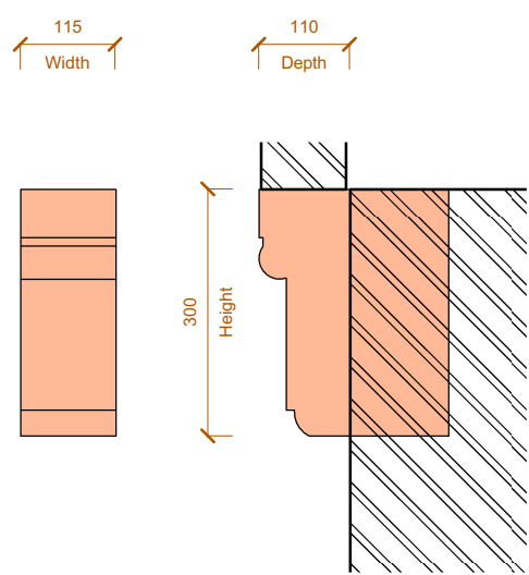
A Proposed Corbel Profile 1 : 10
