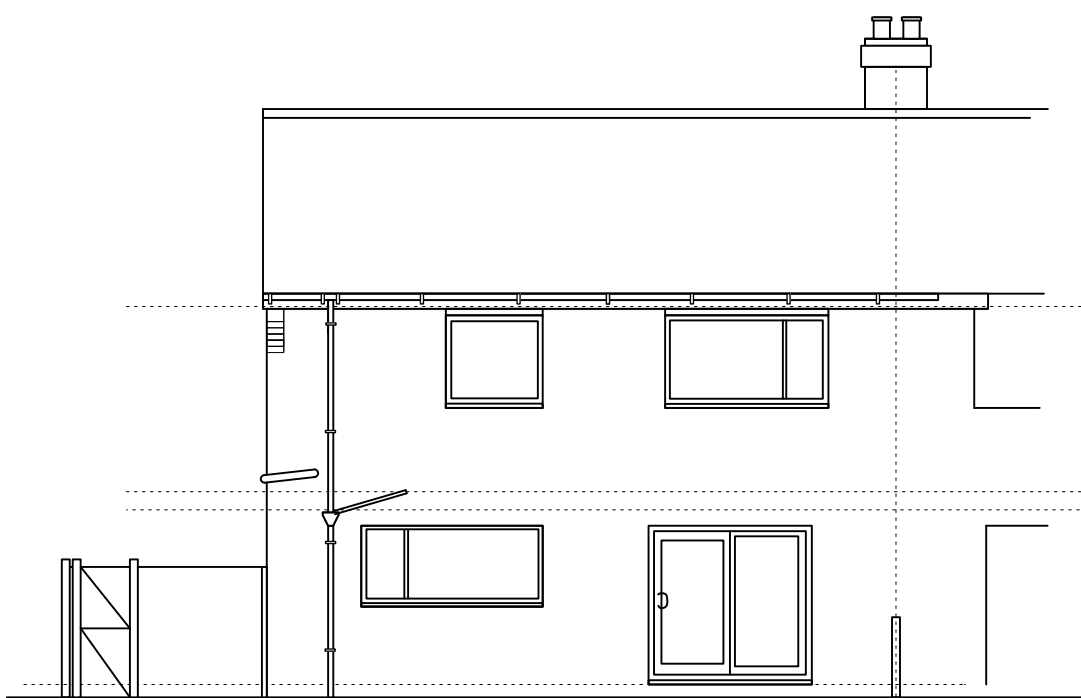
Existing Rear Elevation 1:100 @ A1
