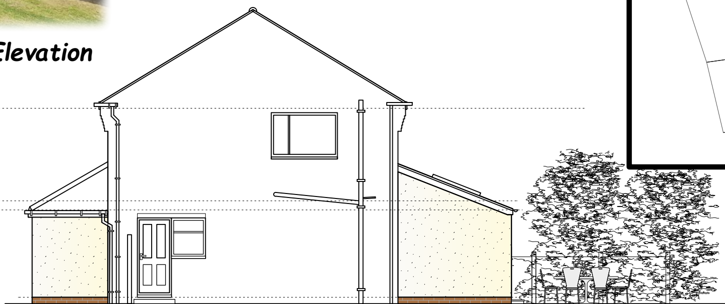
Proposed Side (west) Elevation 1:100 @ A1
