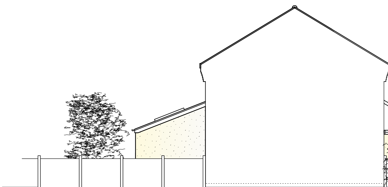
Proposed Side (east - from No 185) Elevation 1:100 @ A1
