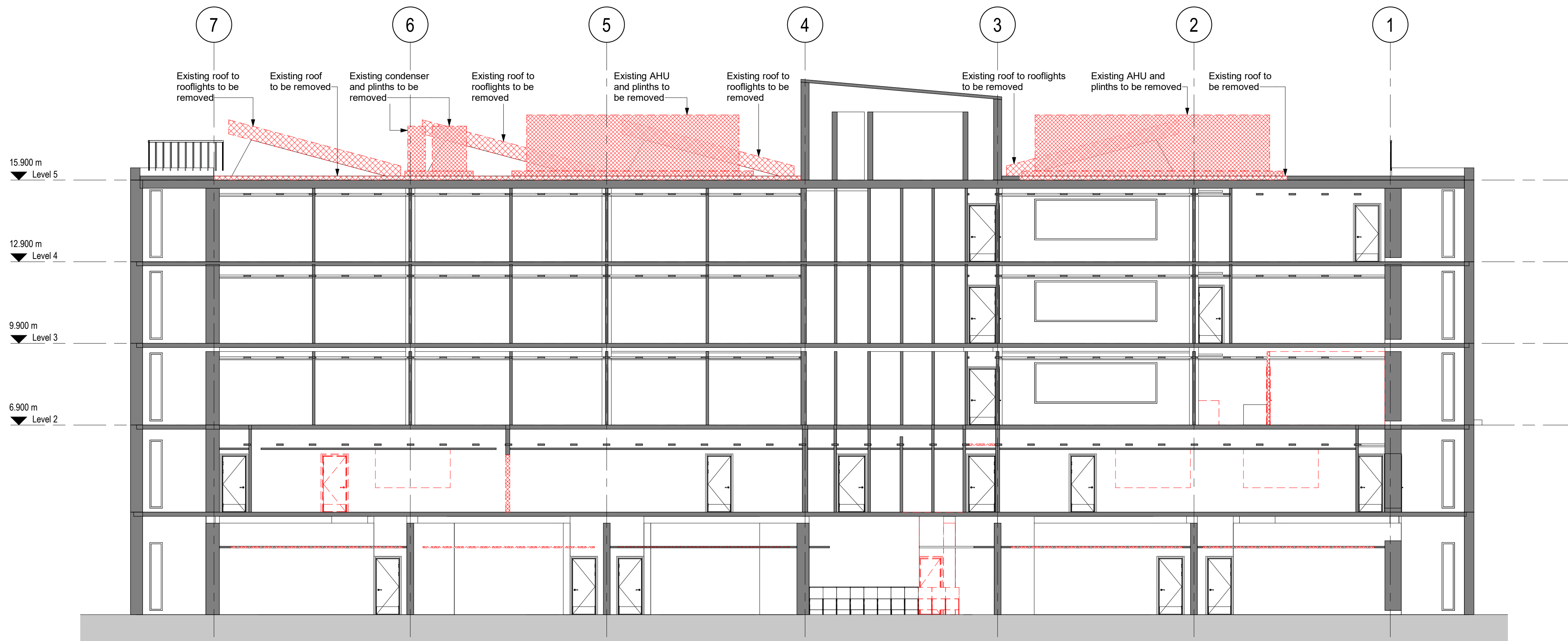
1 Existing section 1: 100 @ A1
