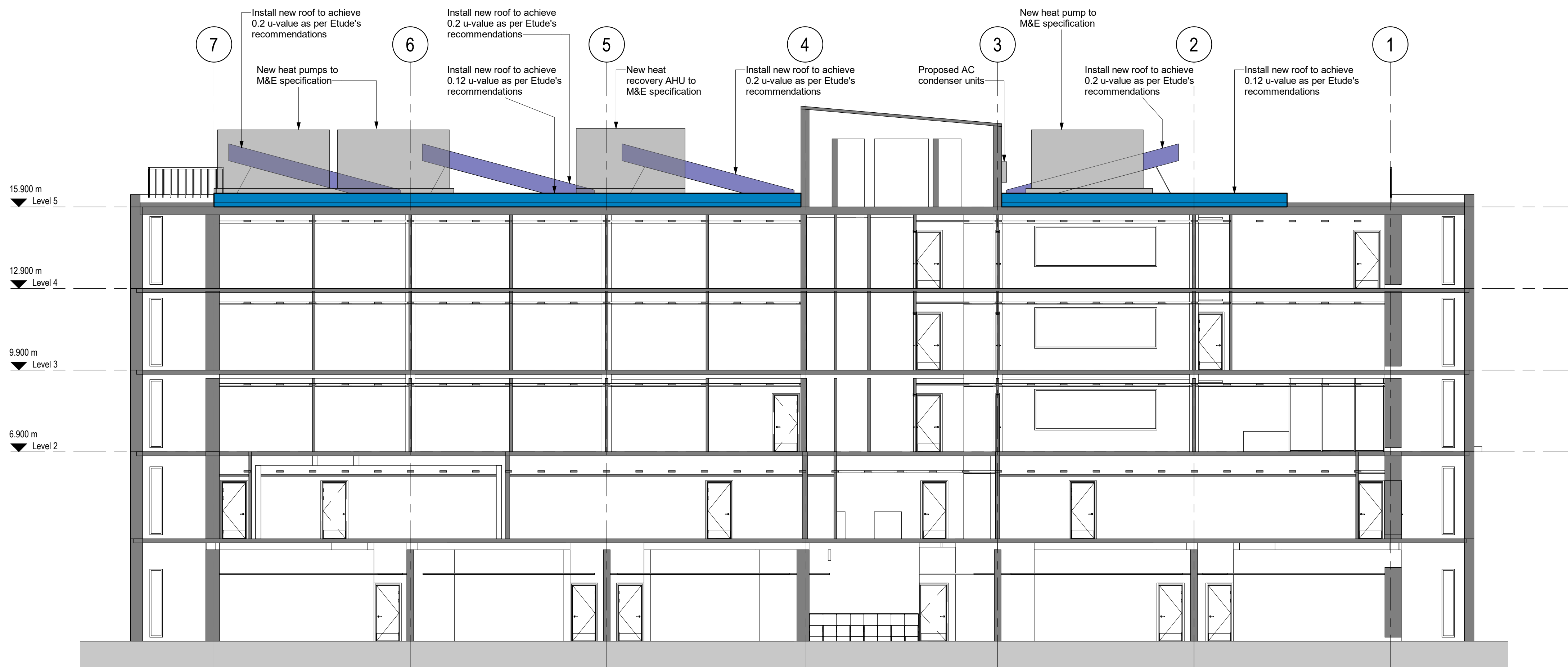
2 Proposed section 1: 100 @ A1
