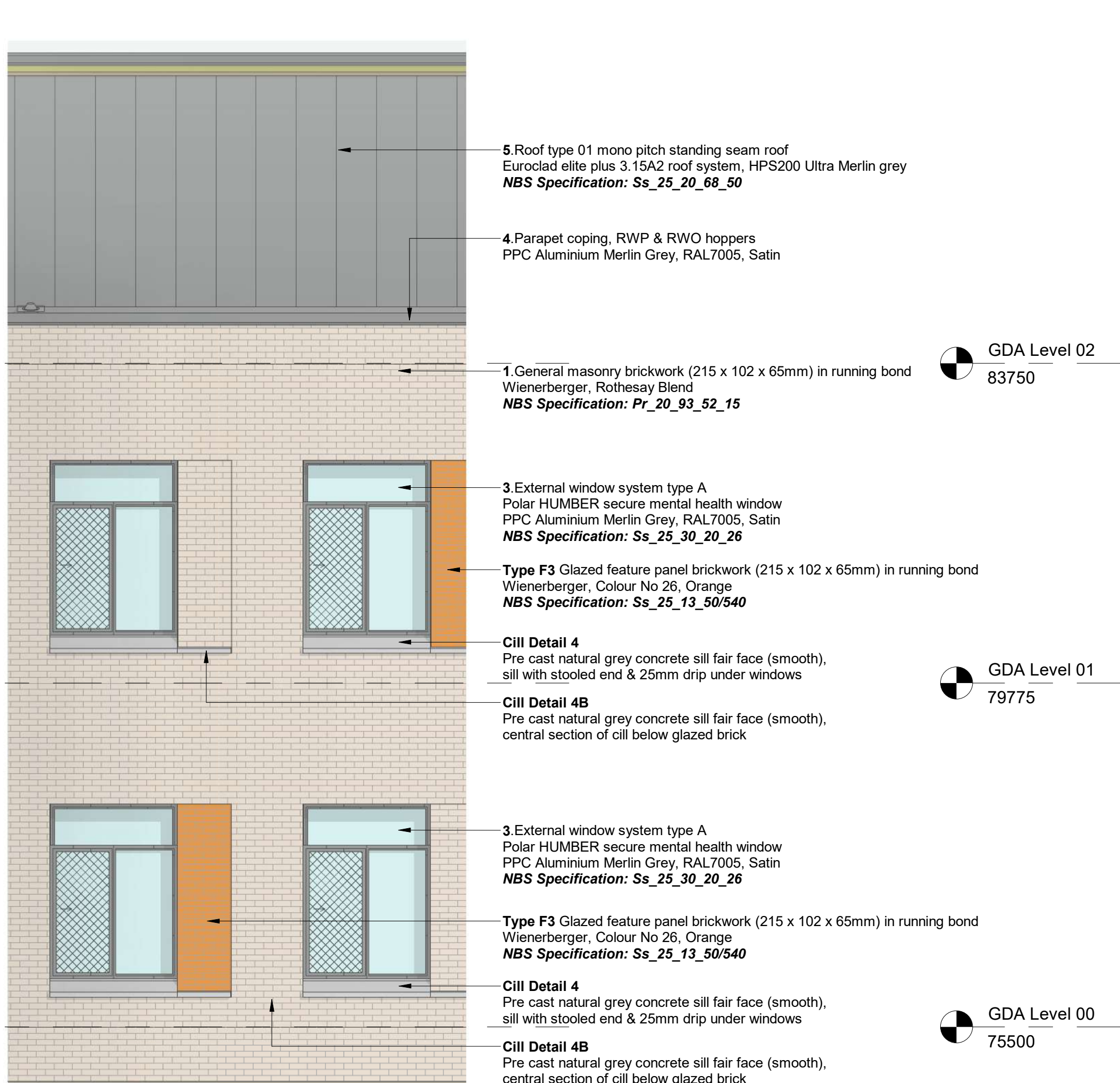
3 Elevation SW2 -V3 Ward 2/ Ward 3 1 : 50
