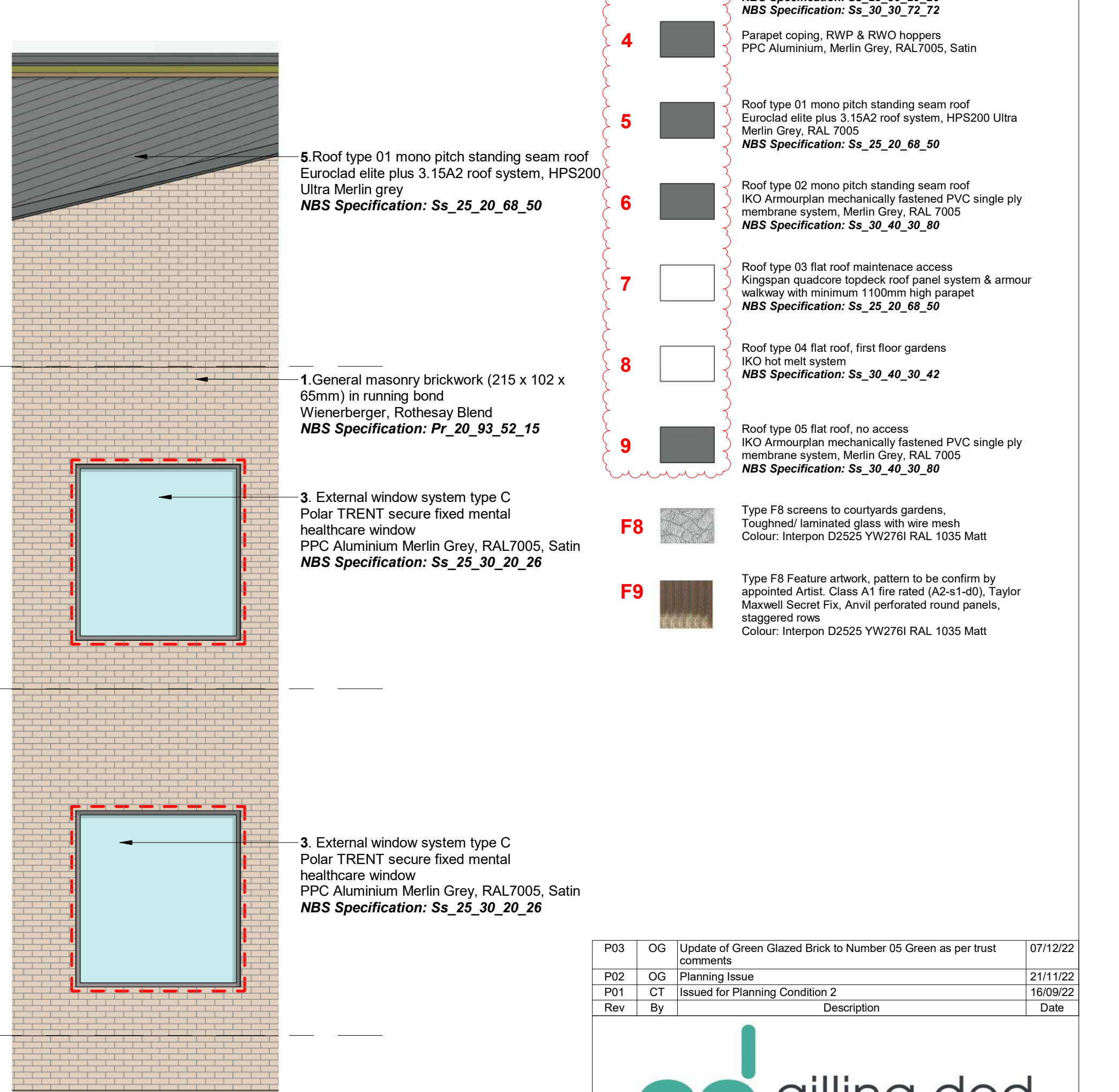
6 Elevation SW2 -Typical Gable End Projecting Window Treatment 1 : 50
