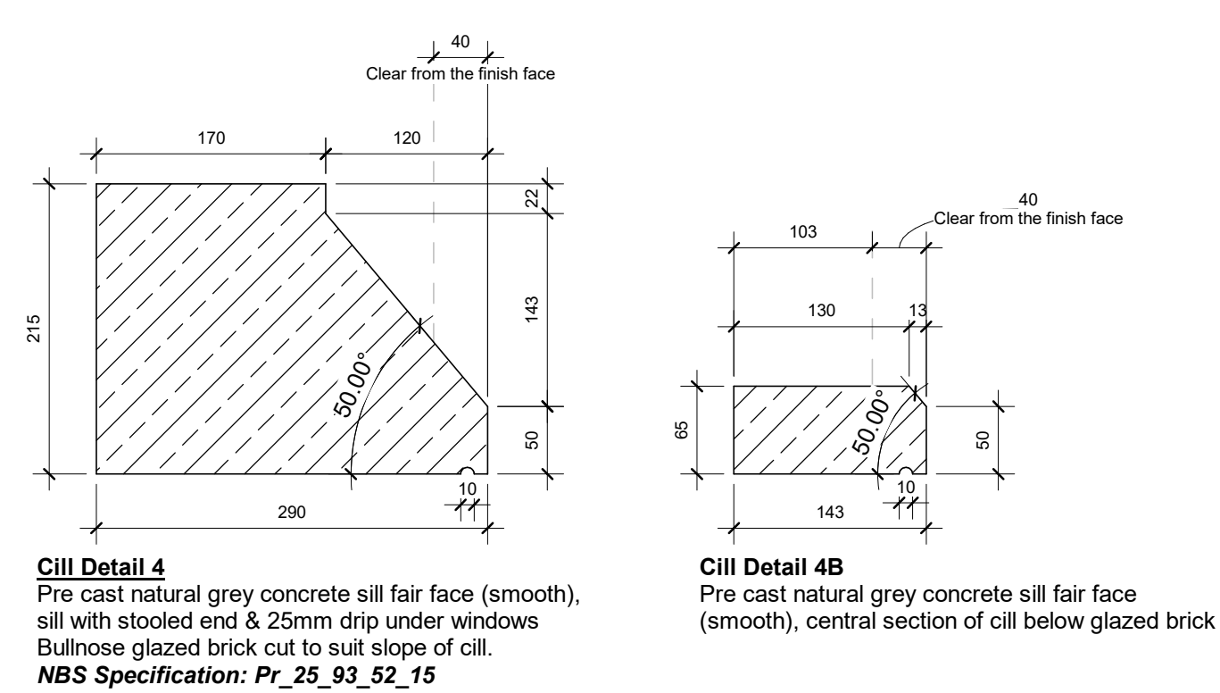
5 Typical Window Cill Details 4 & 4B 1 : 5
