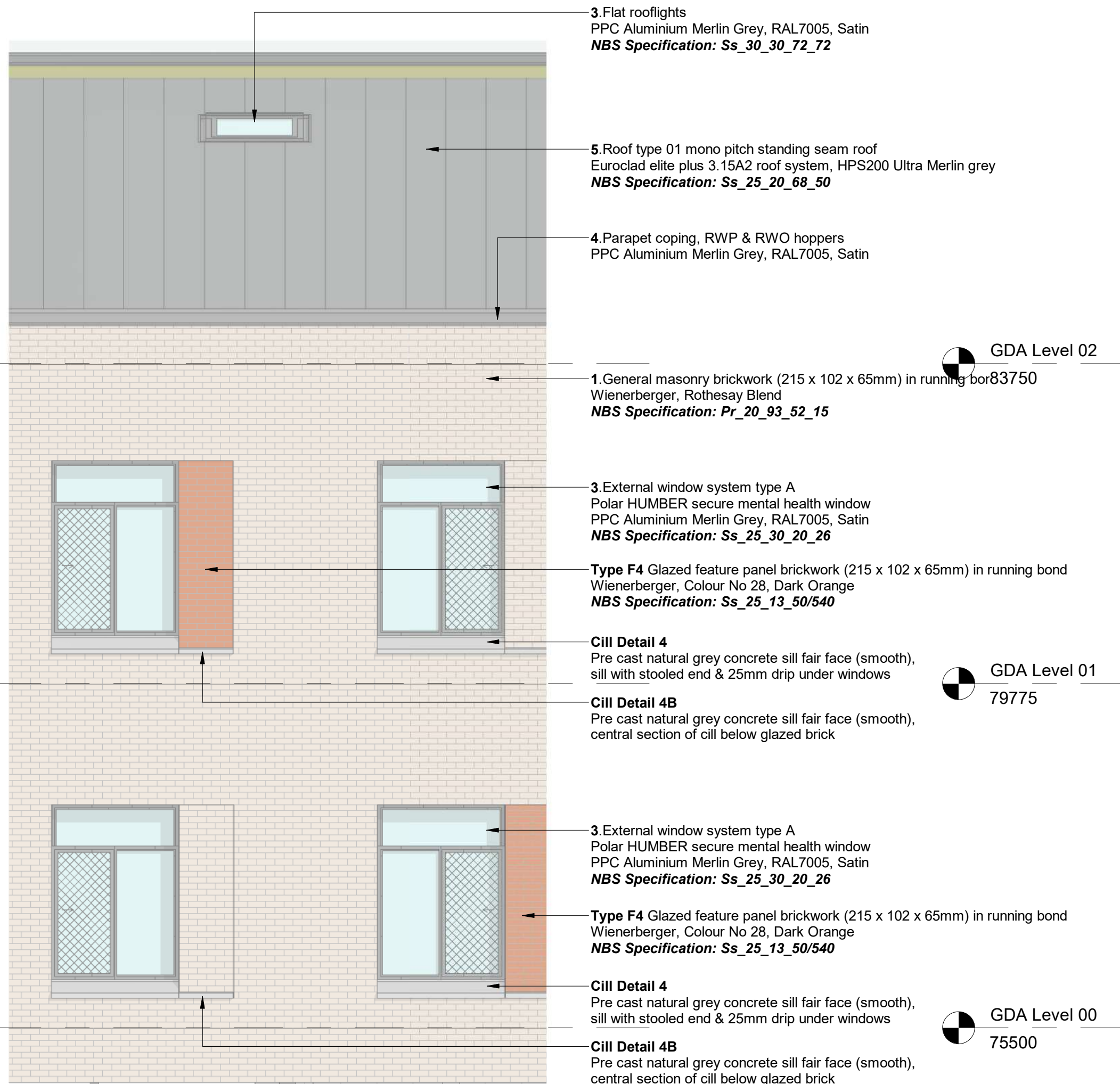
1 Elevation SW2 - Callout 1 1 : 100
