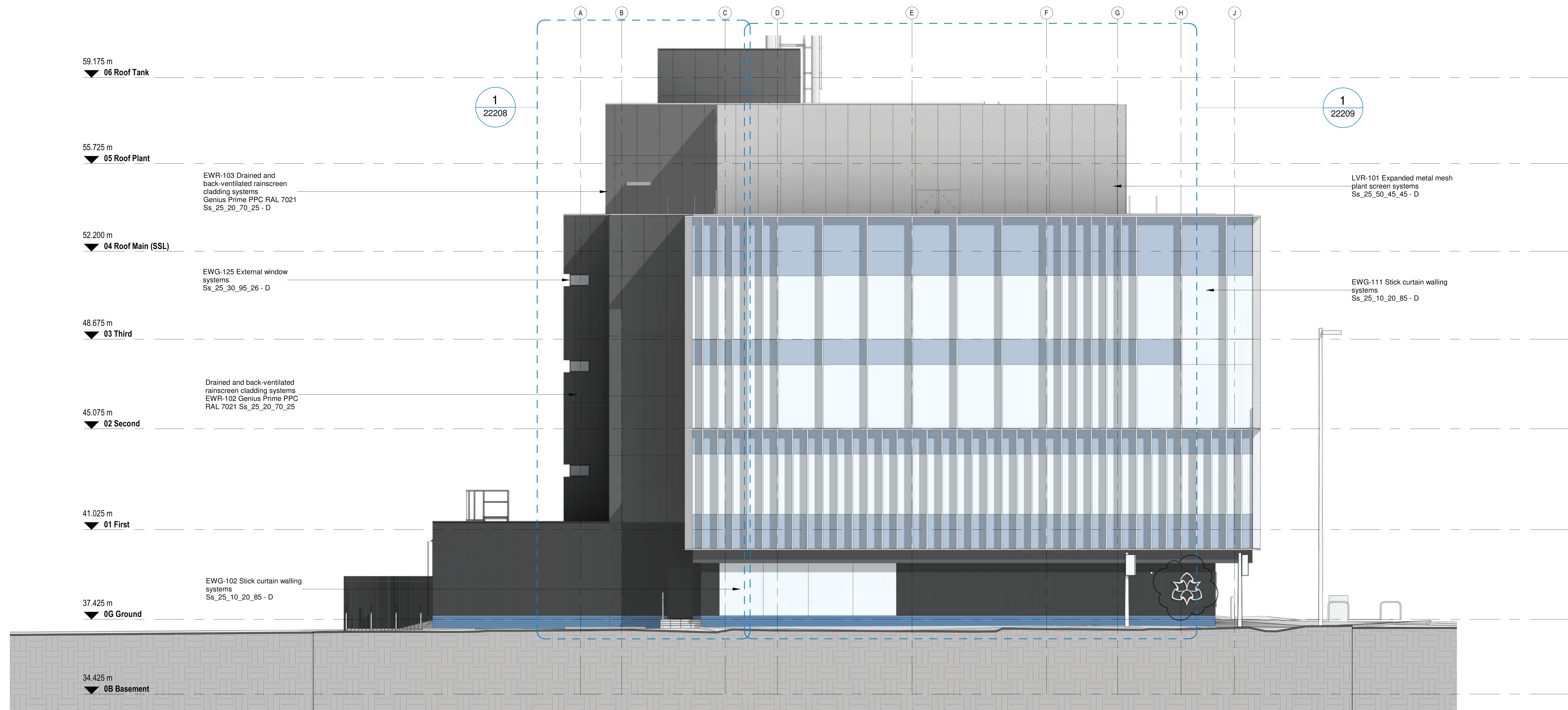
02 GA Elevation - Proposed West Oxford Road 1 : 100
