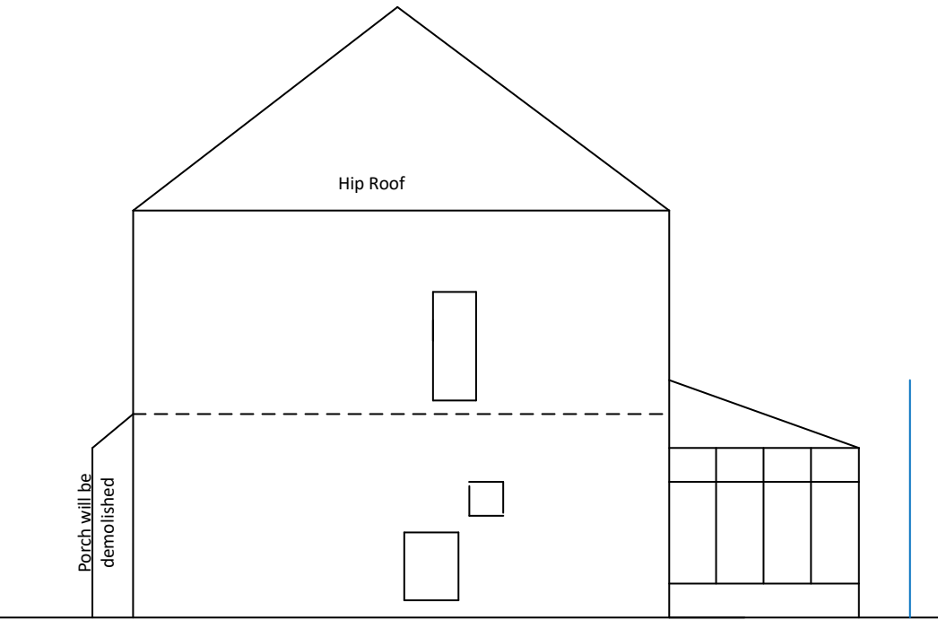
Existing Side Elevation from Smedley Road Side
