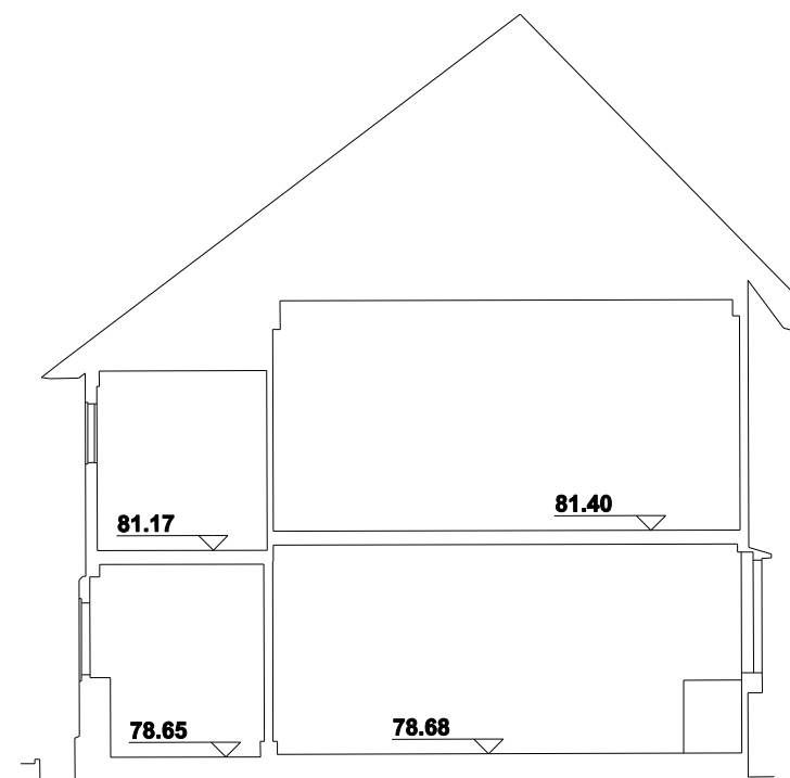
SECTION THROUGH SOUTHERN RANGE
