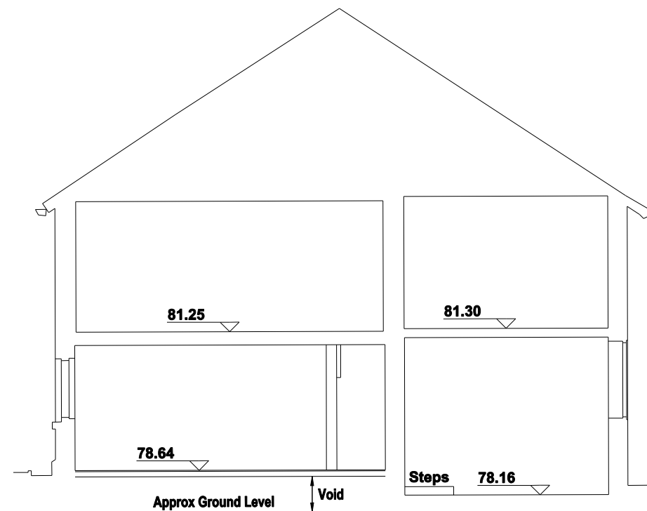
SECTION THROUGH NORTHERN RANGE
