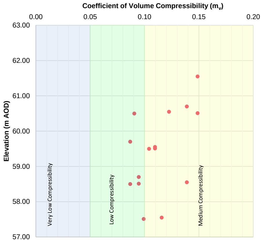
Figure 5.1.2c – Summary of Estimated Coefficient of Volume Compressibility of Cohesive Glacial Till
