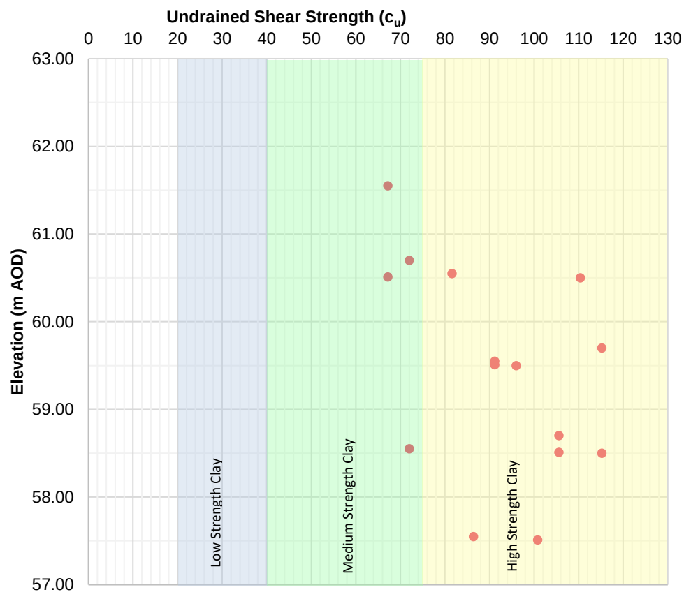
Figure 5.1.2b – Derived Undrained Shear Strength versus Elevation Plot - Cohesive Glacial Till
