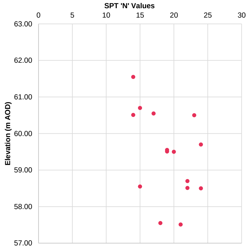
Figure 5.1.2a – SPT 'N' Value versus Elevation (m AOD) – Cohesive Glacial Till
