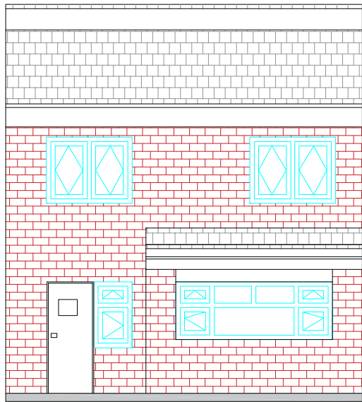
East Elevation
