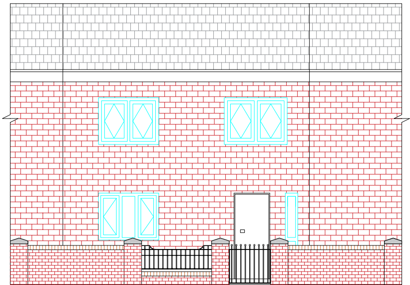
West Elevation
