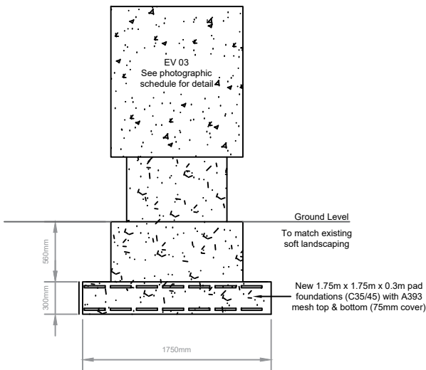
Elevation 03
