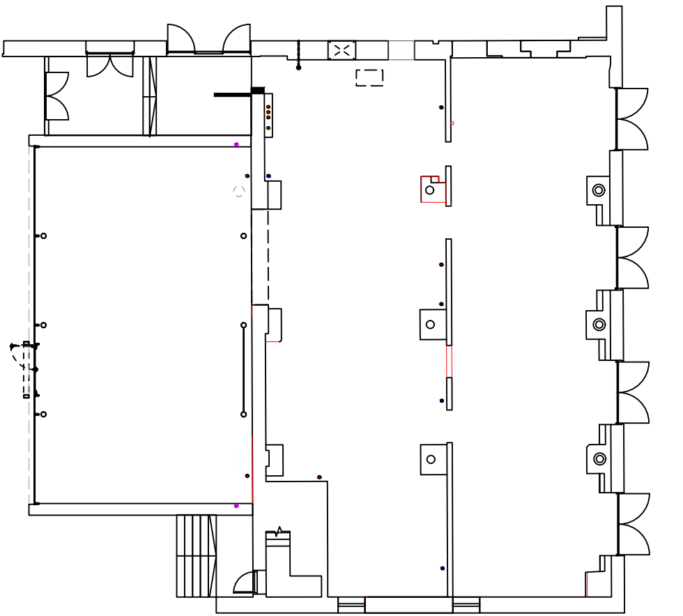
01 030 GROUND FLOOR PLAN AS EXISTING SCALE - 1:200 @ A1 PLAN
