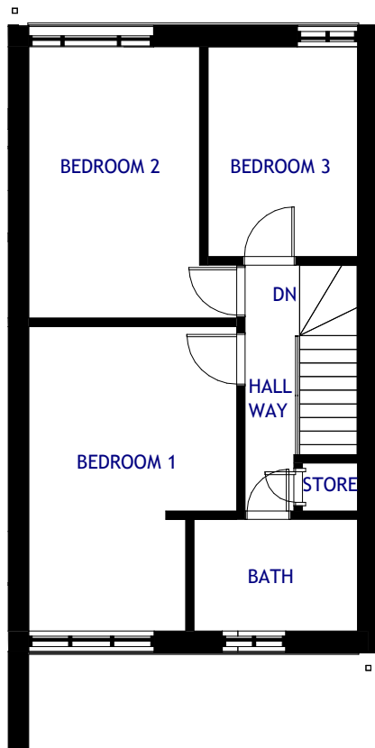
2 First floor Existing 1 : 100
