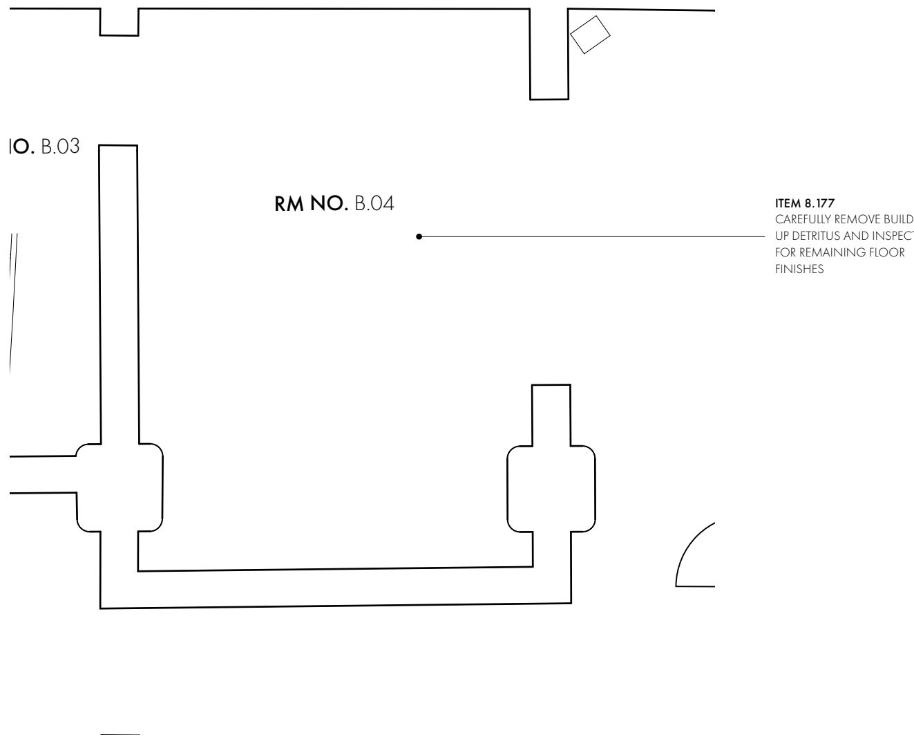
FLOOR FINISHES PLAN
