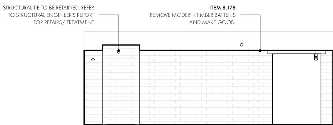
ELEVATION C
