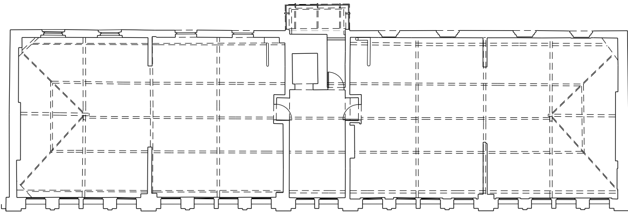
LEVEL 03 EXISTING REFLECTED CEILING PLAN
