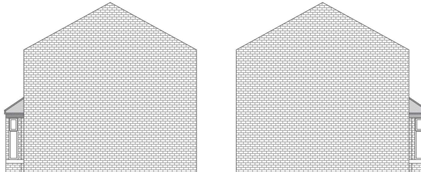
Existing R/H/S elevation
