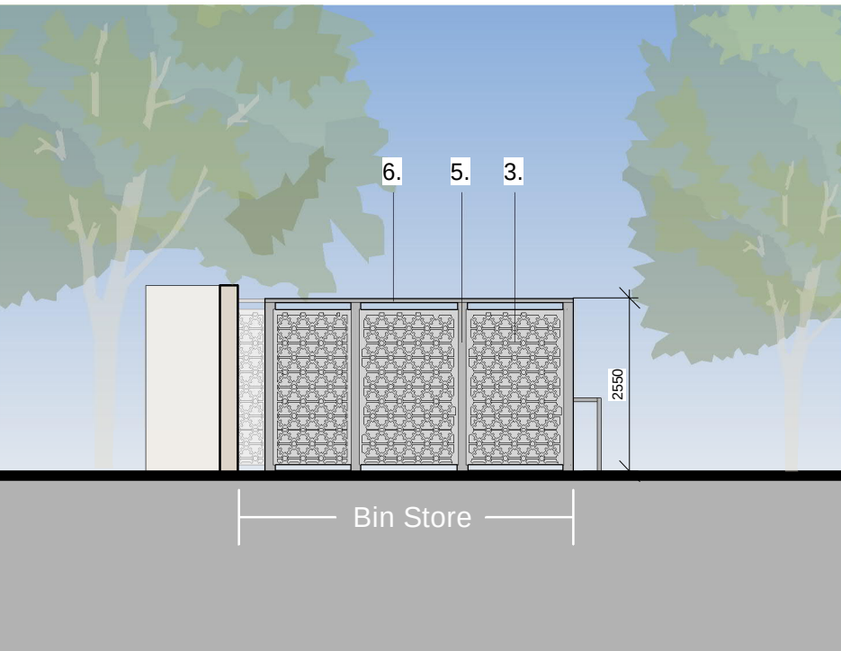
Bin Store - West Elevation 1 : 100
