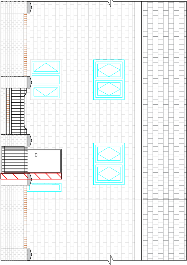
West Elevation
