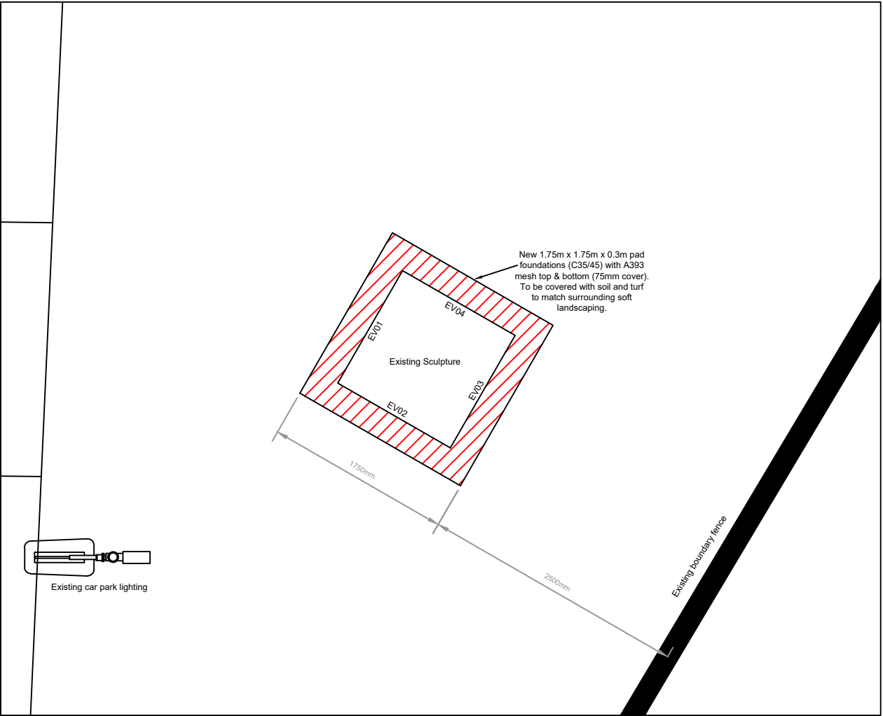
Sculpture Relocation - Proposed Site Plan 1/100
