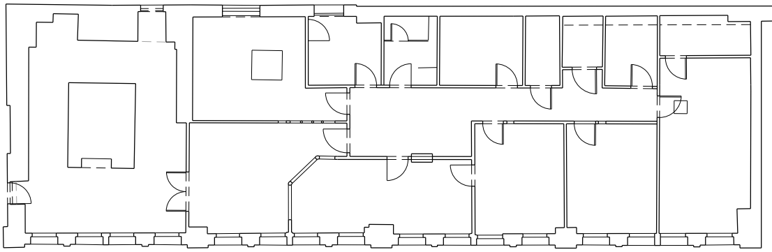
LEVEL 03 EXISTING REFLECTED CEILING PLAN
