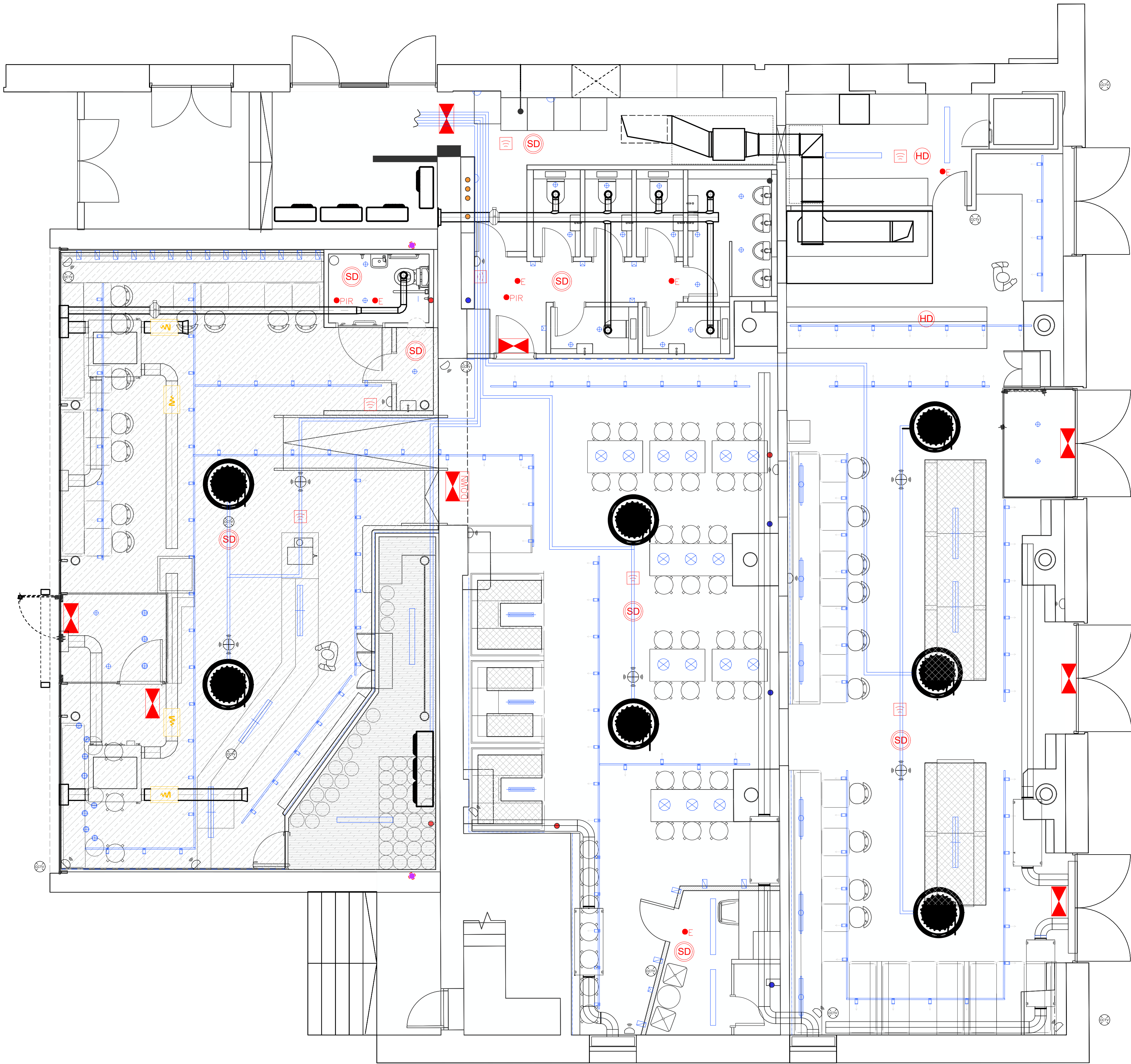
01 RCP AS PROPOSED 300 SCALE - 1:50 @ A1 PLAN
