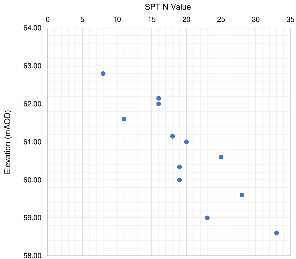
Figure 5.1.2a – SPT 'N' Value versus Elevation (m AOD) – Cohesive Glacial Till
