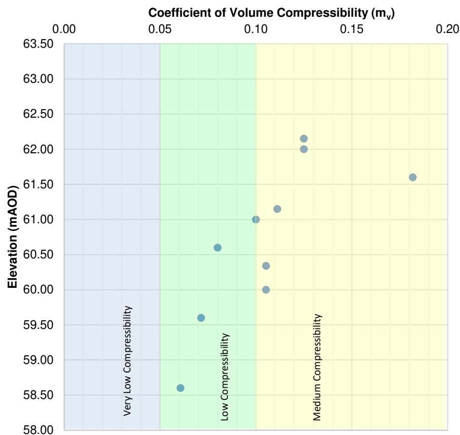
Figure 5.1.2c – Coefficient of Volume Compressibility versus Elevation Plot - Cohesive Glacial Till
