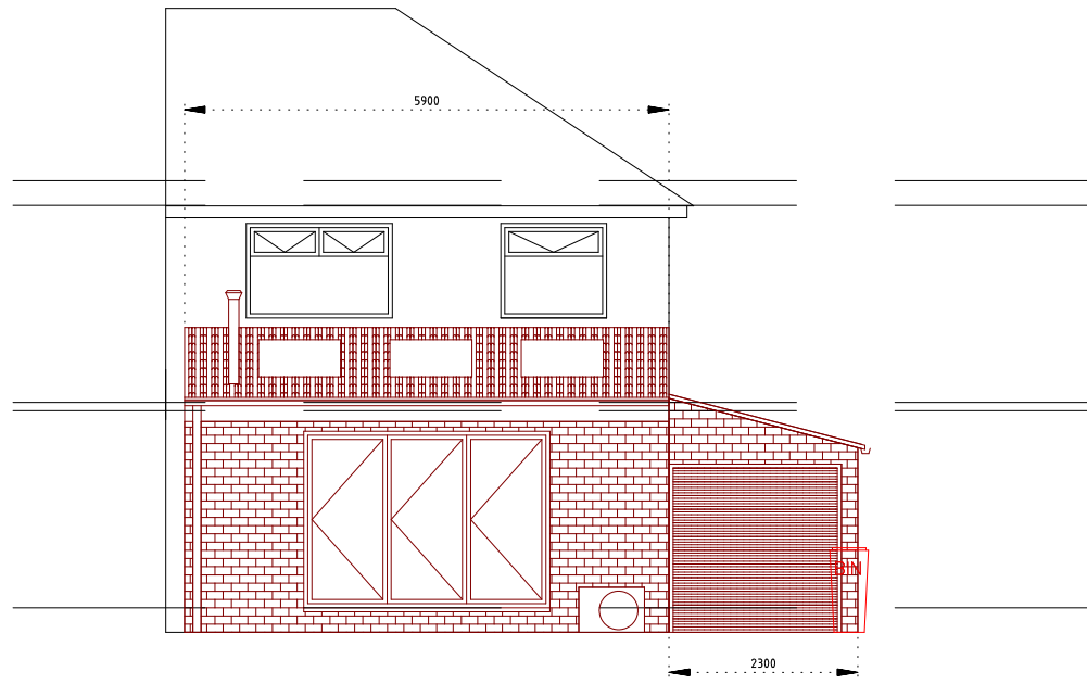
REAR ELEVATION (A3 1:100)
