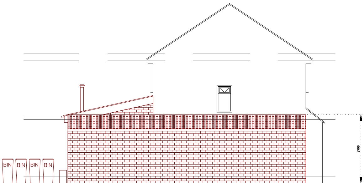
SIDE ELEVATION ELEVATION (from No.6)(A3 1:100)
