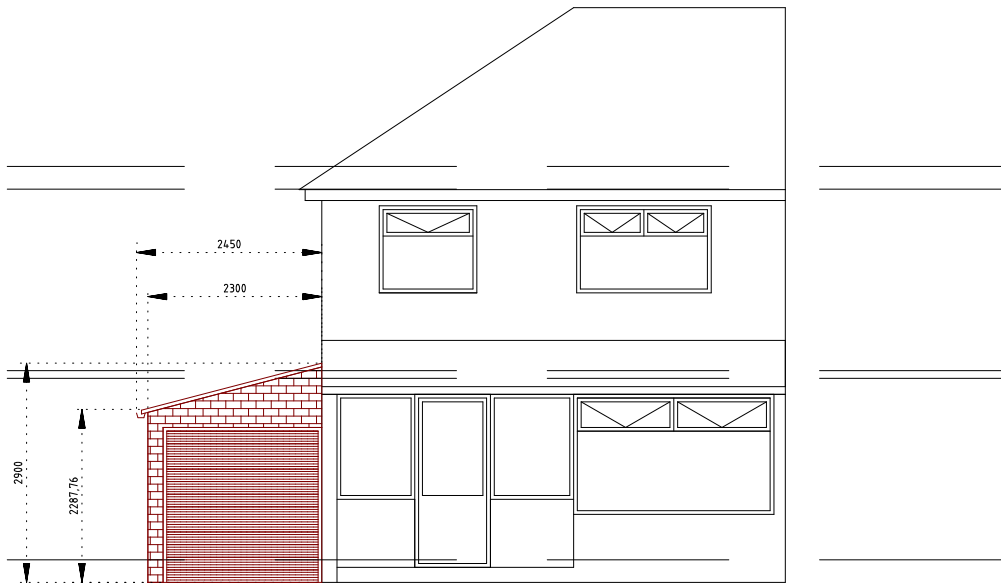
FRONT ELEVATION (A3 1:100)
