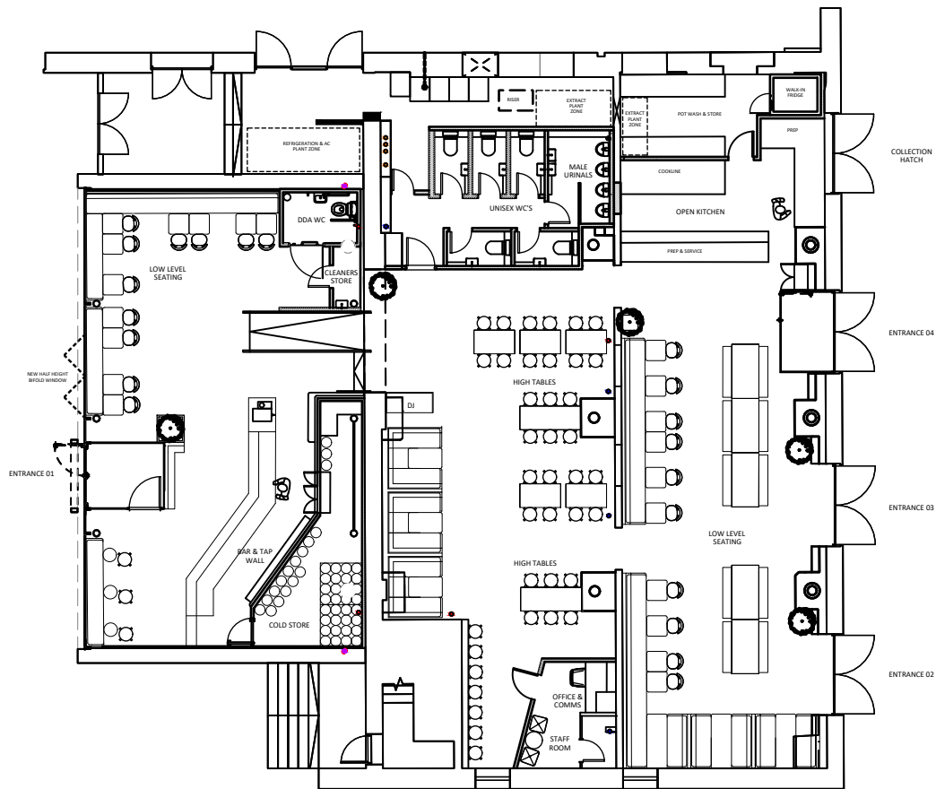
01 GROUND FLOOR PLAN AS PROPOSED 130 SCALE - 1:200 @ A1 PLAN
